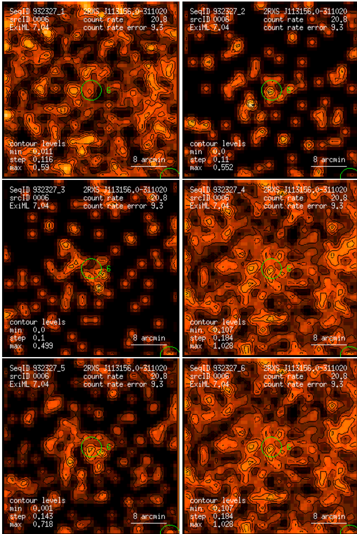
Figure 6: RASS 932327: detection 0006: band rate images, Gaussian filter: (1) PSPC channels 11 – 41, (2) 52 – 90, (3) 91 – 201, (4) 11 – 235, (5) 52 – 201, (6) 11 – 201. Broad band rates in counts/ks. Band rate contour levels in counts/ks/arcmin 2 .
