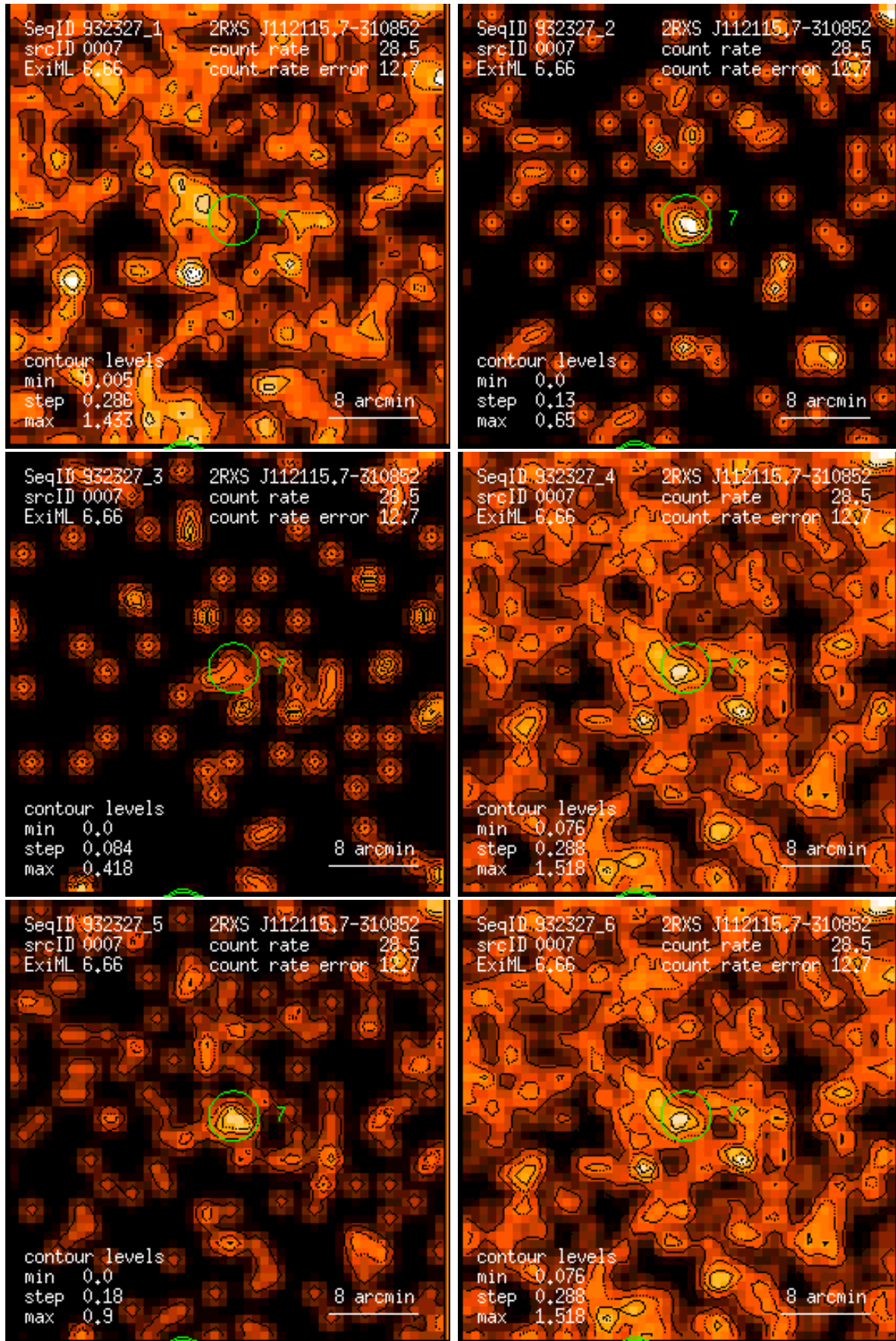
Figure 7: RASS 932327: detection 0007: band rate images, Gaussian filter: (1) PSPC channels 11 – 41, (2) 52 – 90, (3) 91 – 201, (4) 11 – 235, (5) 52 – 201, (6) 11 – 201. Broad band rates in counts/ks. Band rate contour levels in counts/ks/arcmin 2 .
