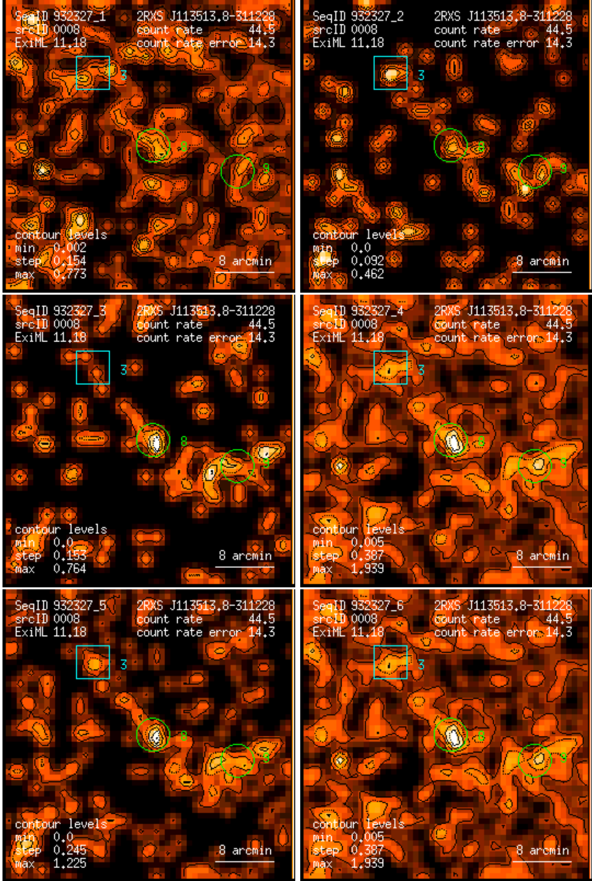
Figure 8: RASS 932327: detection 0008: band rate images, Gaussian filter: (1) PSPC channels 11 – 41, (2) 52 – 90, (3) 91 – 201, (4) 11 – 235, (5) 52 – 201, (6) 11 – 201. Broad band rates in counts/ks. Band rate contour levels in counts/ks/arcmin 2 .
