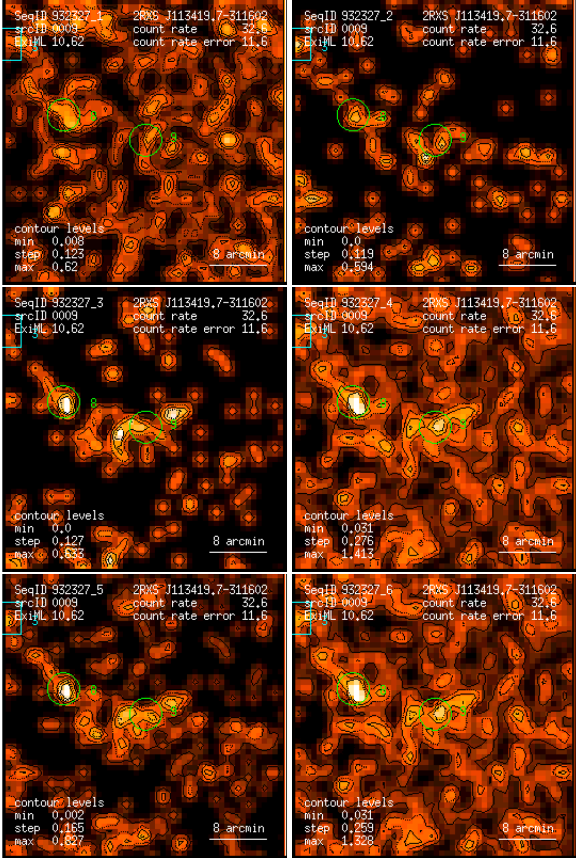
Figure 9: RASS 932327: detection 0009: band rate images, Gaussian filter: (1) PSPC channels 11 – 41, (2) 52 – 90, (3) 91 – 201, (4) 11 – 235, (5) 52 – 201, (6) 11 – 201. Broad band rates in counts/ks. Band rate contour levels in counts/ks/arcmin 2 .
