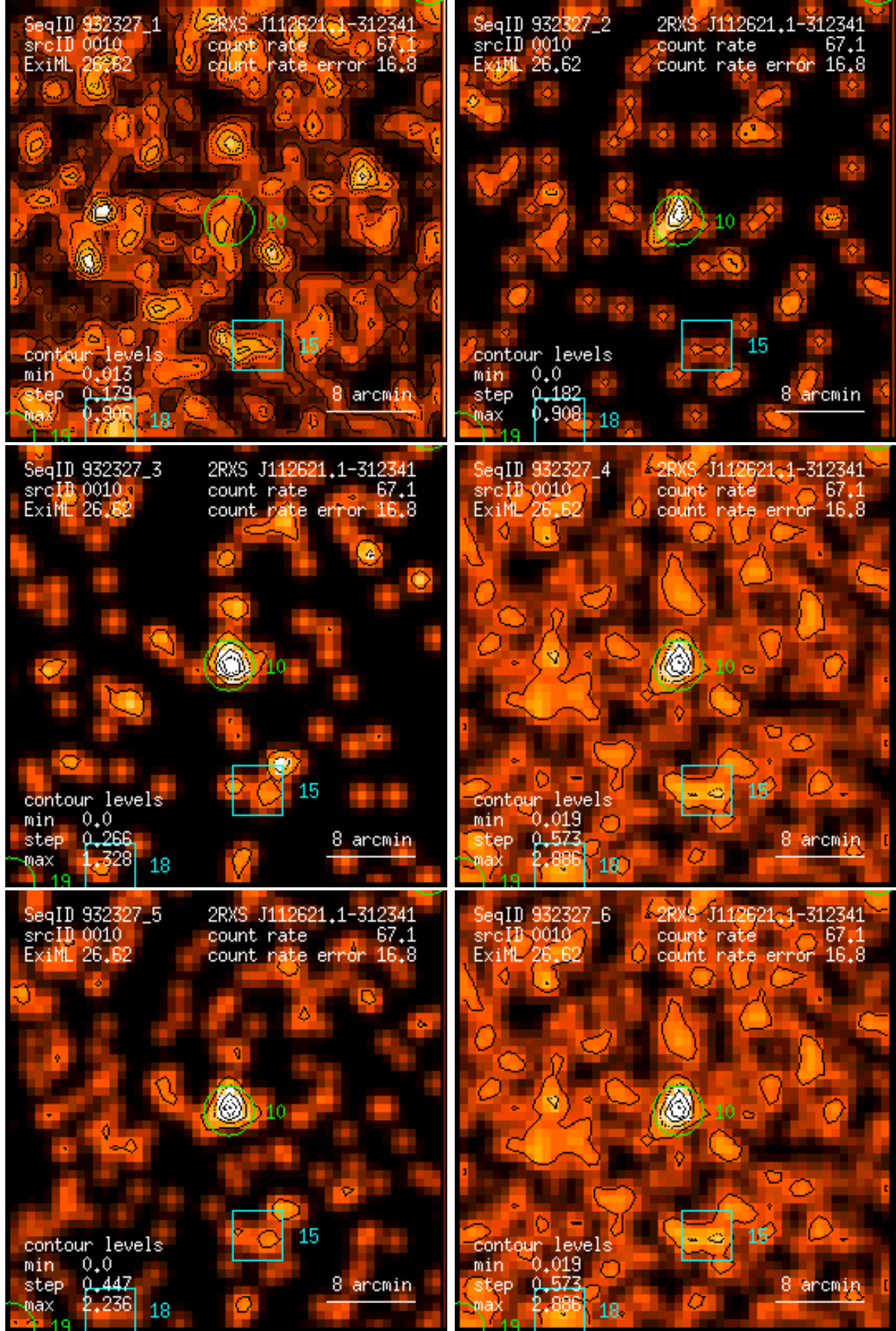
Figure 10: RASS 932327: detection 0010: band rate images, Gaussian filter: (1) PSPC channels 11 – 41, (2) 52 – 90, (3) 91 – 201, (4) 11 – 235, (5) 52 – 201, (6) 11 – 201. Broad band rates in counts/ks. Band rate contour levels in counts/ks/arcmin 2 .
