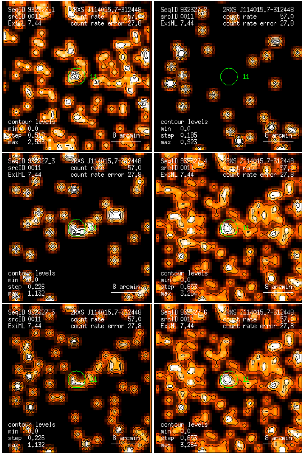
Figure 11: RASS 932327: detection 0011: band rate images, Gaussian filter: (1) PSPC channels 11 – 41, (2) 52 – 90, (3) 91 – 201, (4) 11 – 235, (5) 52 – 201, (6) 11 – 201. Broad band rates in counts/ks. Band rate contour levels in counts/ks/arcmin 2 .
