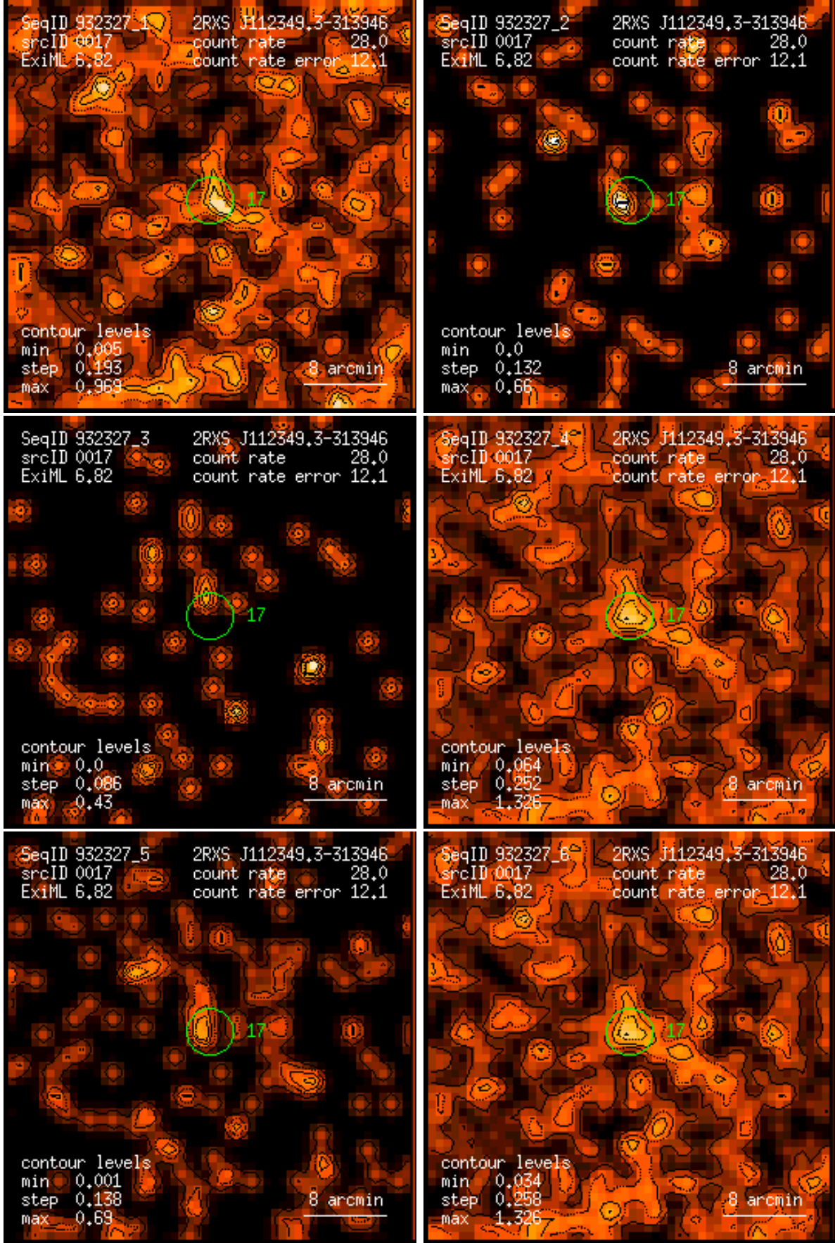
Figure 17: RASS 932327: detection 0017: band rate images, Gaussian filter: (1) PSPC channels 11 – 41, (2) 52 – 90, (3) 91 – 201, (4) 11 – 235, (5) 52 – 201, (6) 11 – 201. Broad band rates in counts/ks. Band rate contour levels in counts/ks/arcmin 2 .
