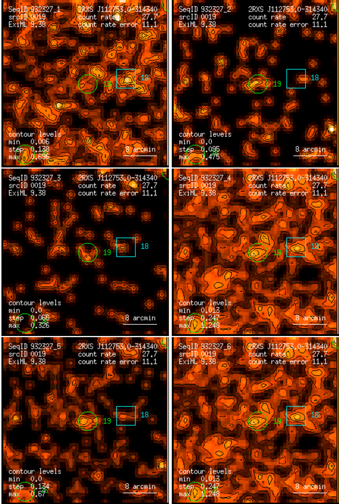
Figure 19: RASS 932327: detection 0019: band rate images, Gaussian filter: (1) PSPC channels 11 – 41, (2) 52 – 90, (3) 91 – 201, (4) 11 – 235, (5) 52 – 201, (6) 11 – 201. Broad band rates in counts/ks. Band rate contour levels in counts/ks/arcmin 2 .
