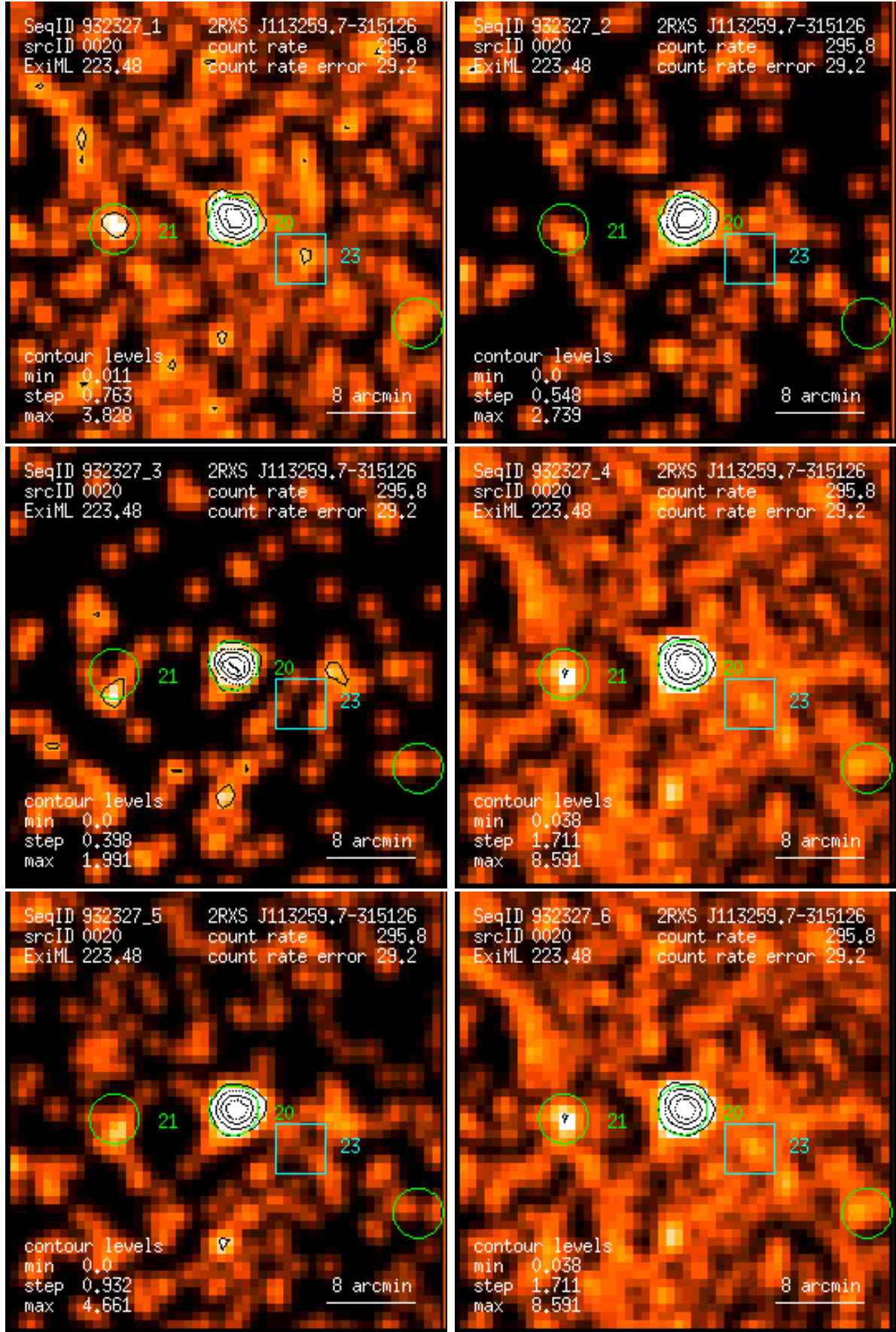
Figure 20: RASS 932327: detection 0020: band rate images, Gaussian filter: (1) PSPC channels 11 – 41, (2) 52 – 90, (3) 91 – 201, (4) 11 – 235, (5) 52 – 201, (6) 11 – 201. Broad band rates in counts/ks. Band rate contour levels in counts/ks/arcmin 2 .
