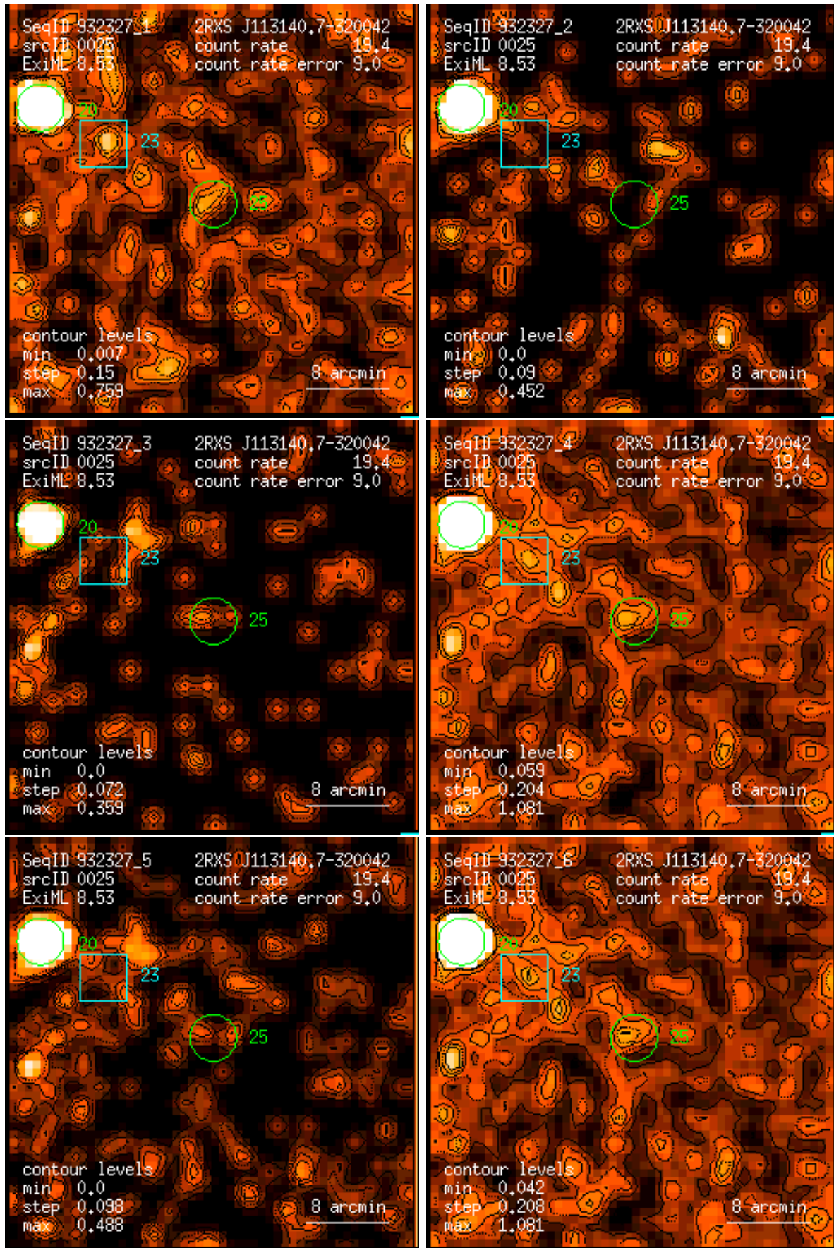
Figure 25: RASS 932327: detection 0025: band rate images, Gaussian filter: (1) PSPC channels 11 – 41, (2) 52 – 90, (3) 91 – 201, (4) 11 – 235, (5) 52 – 201, (6) 11 – 201. Broad band rates in counts/ks. Band rate contour levels in counts/ks/arcmin 2 .
