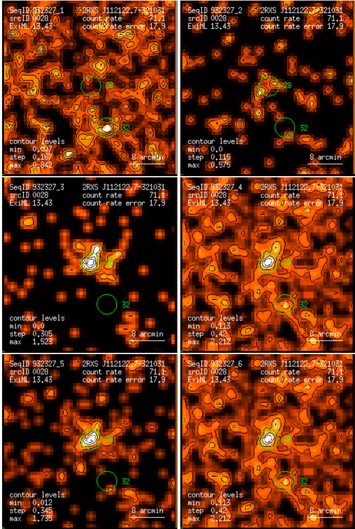
Figure 28: RASS 932327: detection 0028: band rate images, Gaussian filter: (1) PSPC channels 11 – 41, (2) 52 – 90, (3) 91 – 201, (4) 11 – 235, (5) 52 – 201, (6) 11 – 201. Broad band rates in counts/ks. Band rate contour levels in counts/ks/arcmin 2 .
