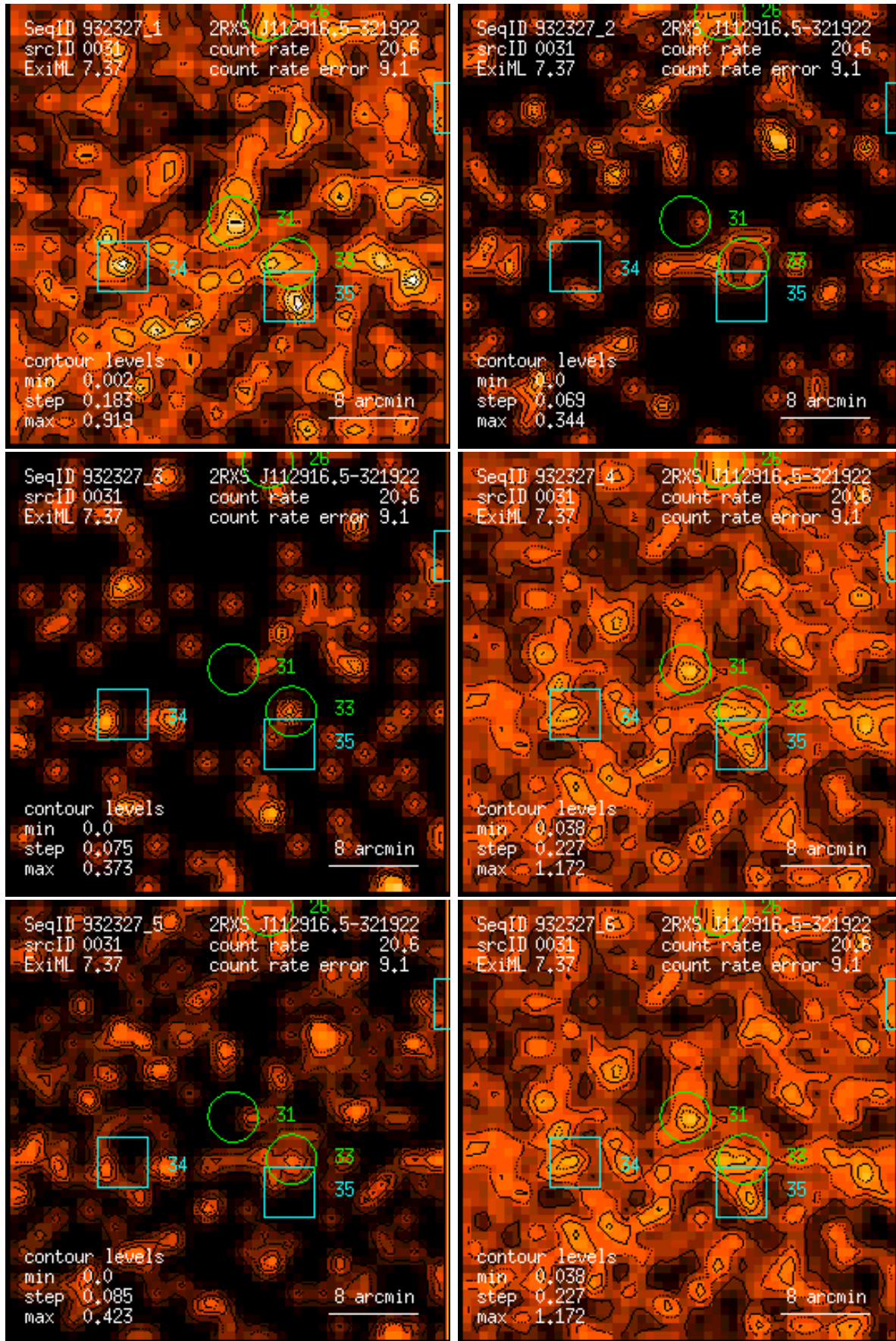
Figure 31: RASS 932327: detection 0031: band rate images, Gaussian filter: (1) PSPC channels 11 – 41, (2) 52 – 90, (3) 91 – 201, (4) 11 – 235, (5) 52 – 201, (6) 11 – 201. Broad band rates in counts/ks. Band rate contour levels in counts/ks/arcmin 2 .
