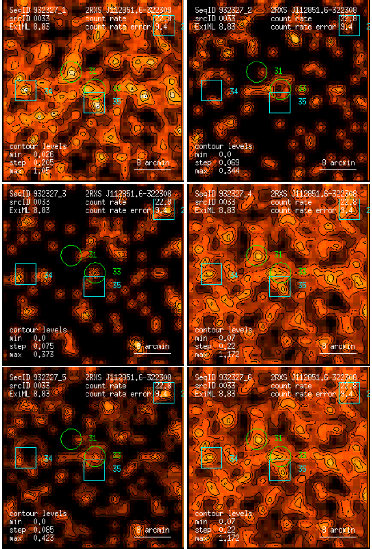
Figure 33: RASS 932327: detection 0033: band rate images, Gaussian filter: (1) PSPC channels 11 – 41, (2) 52 – 90, (3) 91 – 201, (4) 11 – 235, (5) 52 – 201, (6) 11 – 201. Broad band rates in counts/ks. Band rate contour levels in counts/ks/arcmin 2 .
