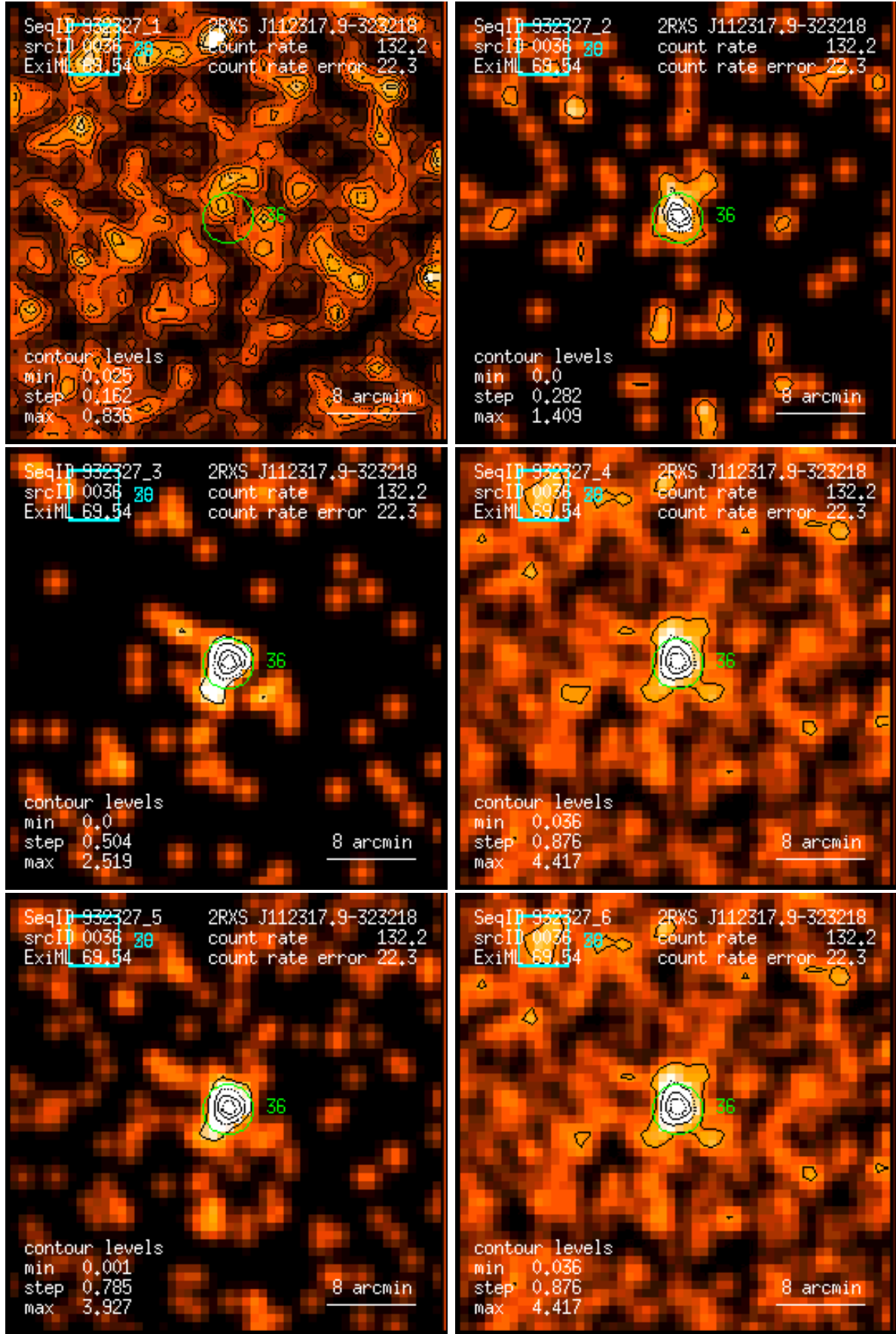
Figure 36: RASS 932327: detection 0036: band rate images, Gaussian filter: (1) PSPC channels 11 – 41, (2) 52 – 90, (3) 91 – 201, (4) 11 – 235, (5) 52 – 201, (6) 11 – 201. Broad band rates in counts/ks. Band rate contour levels in counts/ks/arcmin 2 .
