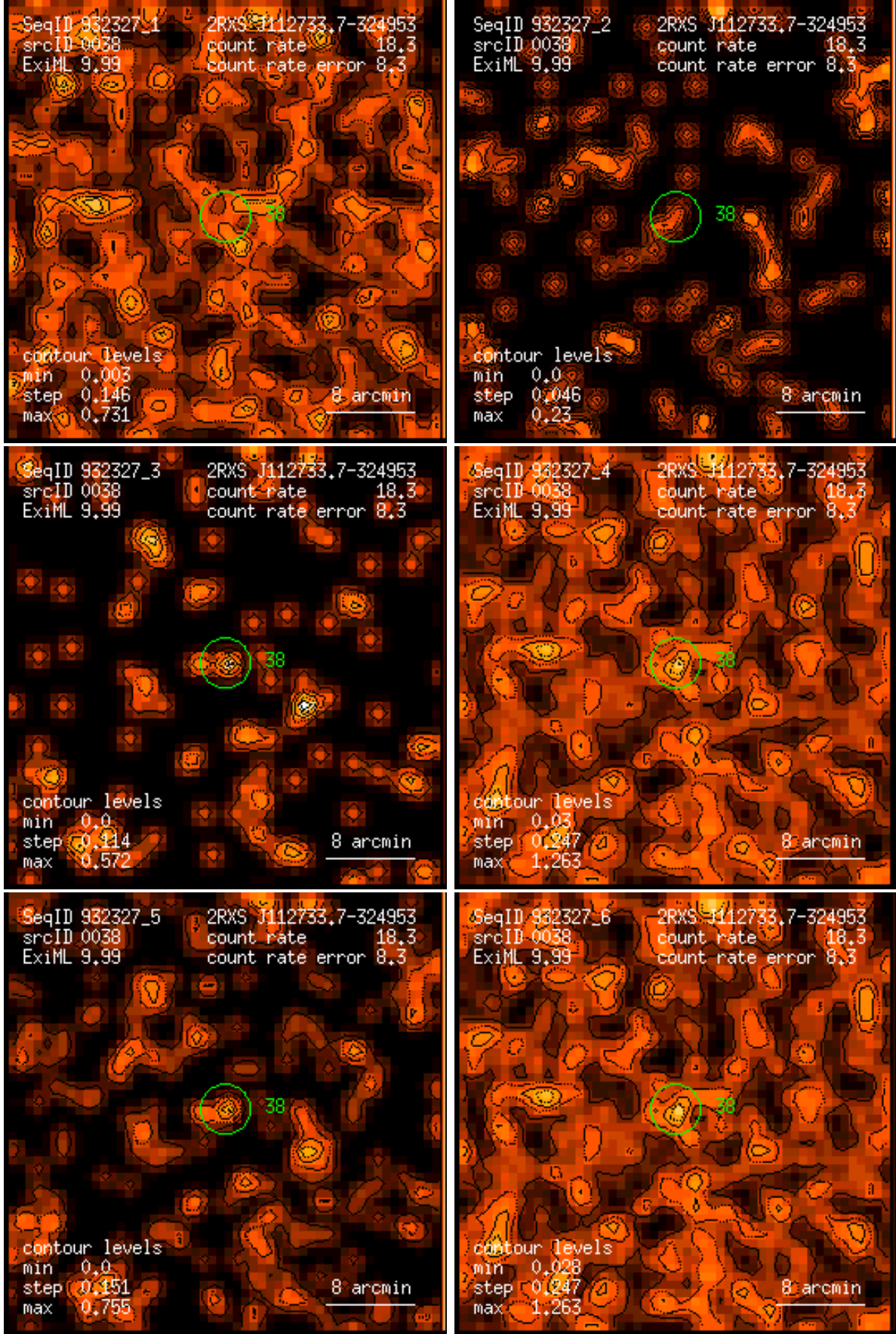
Figure 38: RASS 932327: detection 0038: band rate images, Gaussian filter: (1) PSPC channels 11 – 41, (2) 52 – 90, (3) 91 – 201, (4) 11 – 235, (5) 52 – 201, (6) 11 – 201. Broad band rates in counts/ks. Band rate contour levels in counts/ks/arcmin 2 .
