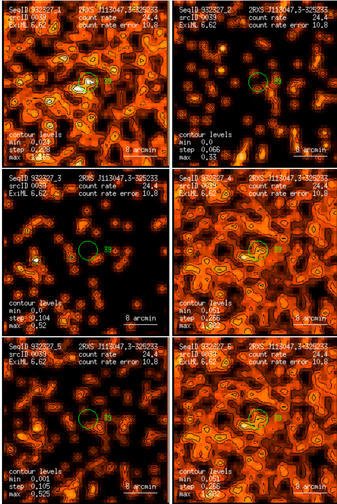
Figure 39: RASS 932327: detection 0039: band rate images, Gaussian filter: (1) PSPC channels 11 – 41, (2) 52 – 90, (3) 91 – 201, (4) 11 – 235, (5) 52 – 201, (6) 11 – 201. Broad band rates in counts/ks. Band rate contour levels in counts/ks/arcmin 2 .
