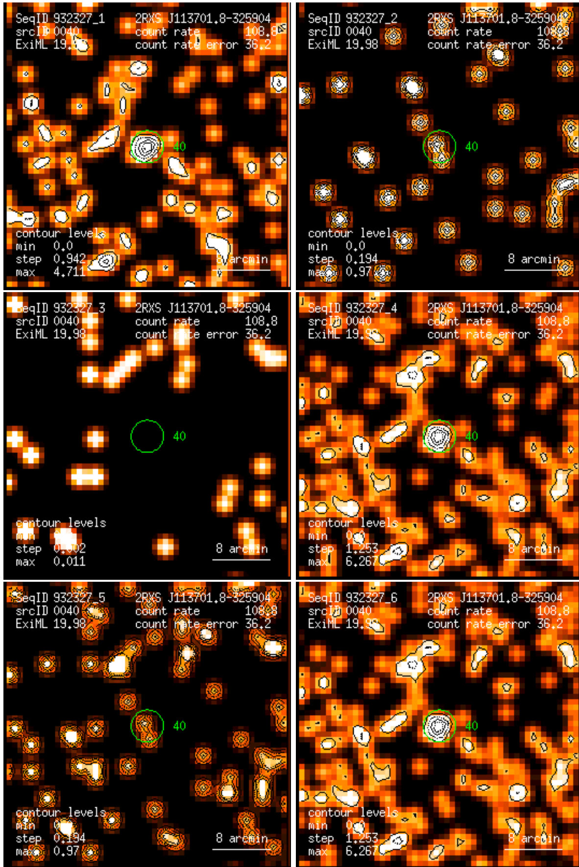
Figure 40: RASS 932327: detection 0040: band rate images, Gaussian filter: (1) PSPC channels 11 – 41, (2) 52 – 90, (3) 91 – 201, (4) 11 – 235, (5) 52 – 201, (6) 11 – 201. Broad band rates in counts/ks. Band rate contour levels in counts/ks/arcmin 2 .
