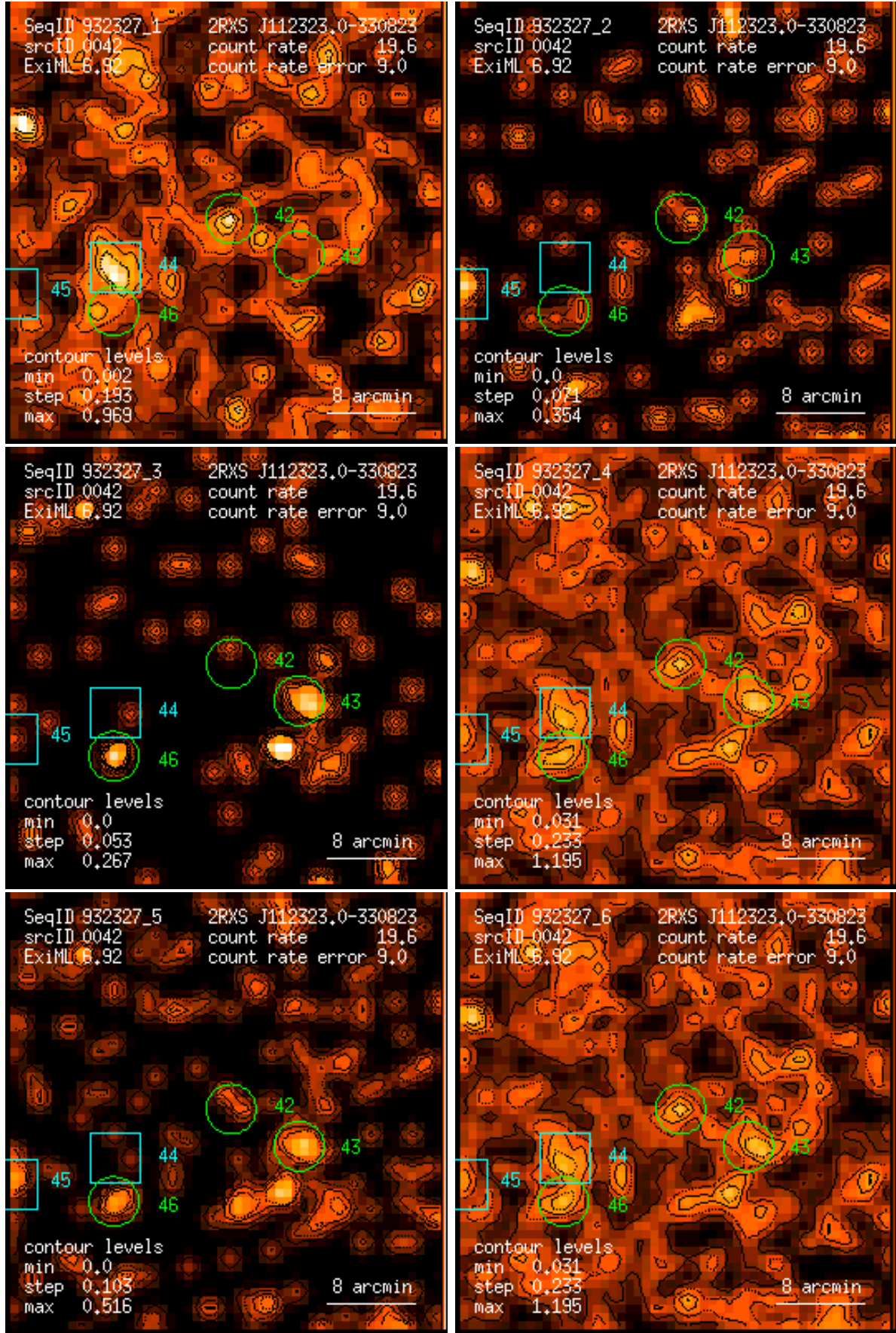
Figure 42: RASS 932327: detection 0042: band rate images, Gaussian filter: (1) PSPC channels 11 – 41, (2) 52 – 90, (3) 91 – 201, (4) 11 – 235, (5) 52 – 201, (6) 11 – 201. Broad band rates in counts/ks. Band rate contour levels in counts/ks/arcmin 2 .
