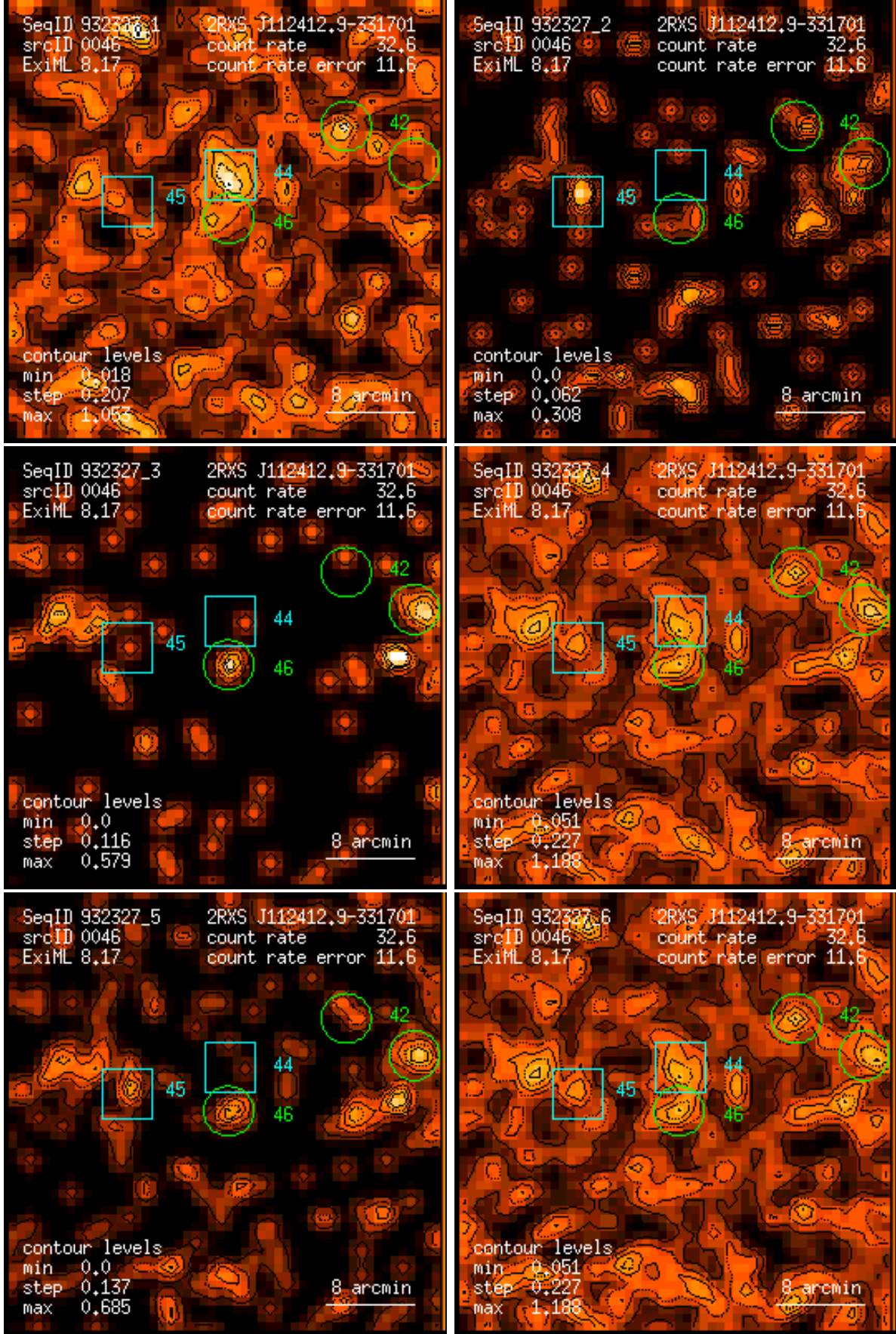
Figure 46: RASS 932327: detection 0046: band rate images, Gaussian filter: (1) PSPC channels 11 – 41, (2) 52 – 90, (3) 91 – 201, (4) 11 – 235, (5) 52 – 201, (6) 11 – 201. Broad band rates in counts/ks. Band rate contour levels in counts/ks/arcmin 2 .
