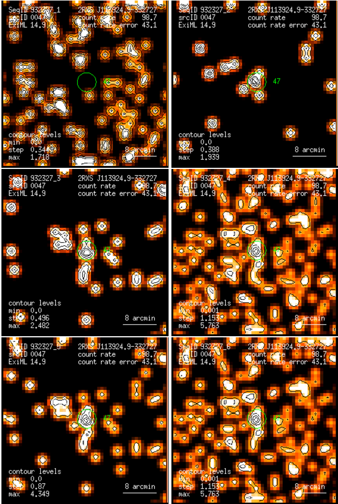
Figure 47: RASS 932327: detection 0047: band rate images, Gaussian filter: (1) PSPC channels 11 – 41, (2) 52 – 90, (3) 91 – 201, (4) 11 – 235, (5) 52 – 201, (6) 11 – 201. Broad band rates in counts/ks. Band rate contour levels in counts/ks/arcmin 2 .
