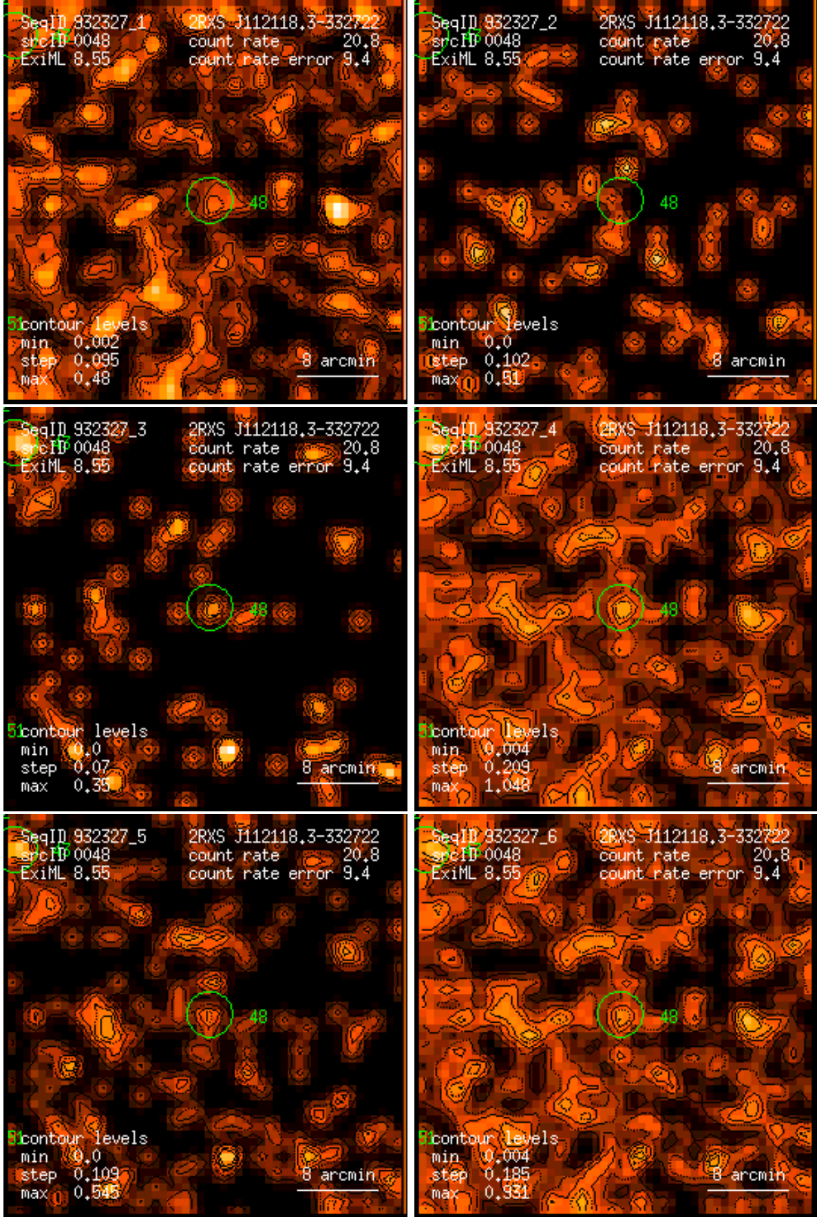
Figure 48: RASS 932327: detection 0048: band rate images, Gaussian filter: (1) PSPC channels 11 – 41, (2) 52 – 90, (3) 91 – 201, (4) 11 – 235, (5) 52 – 201, (6) 11 – 201. Broad band rates in counts/ks. Band rate contour levels in counts/ks/arcmin 2 .
