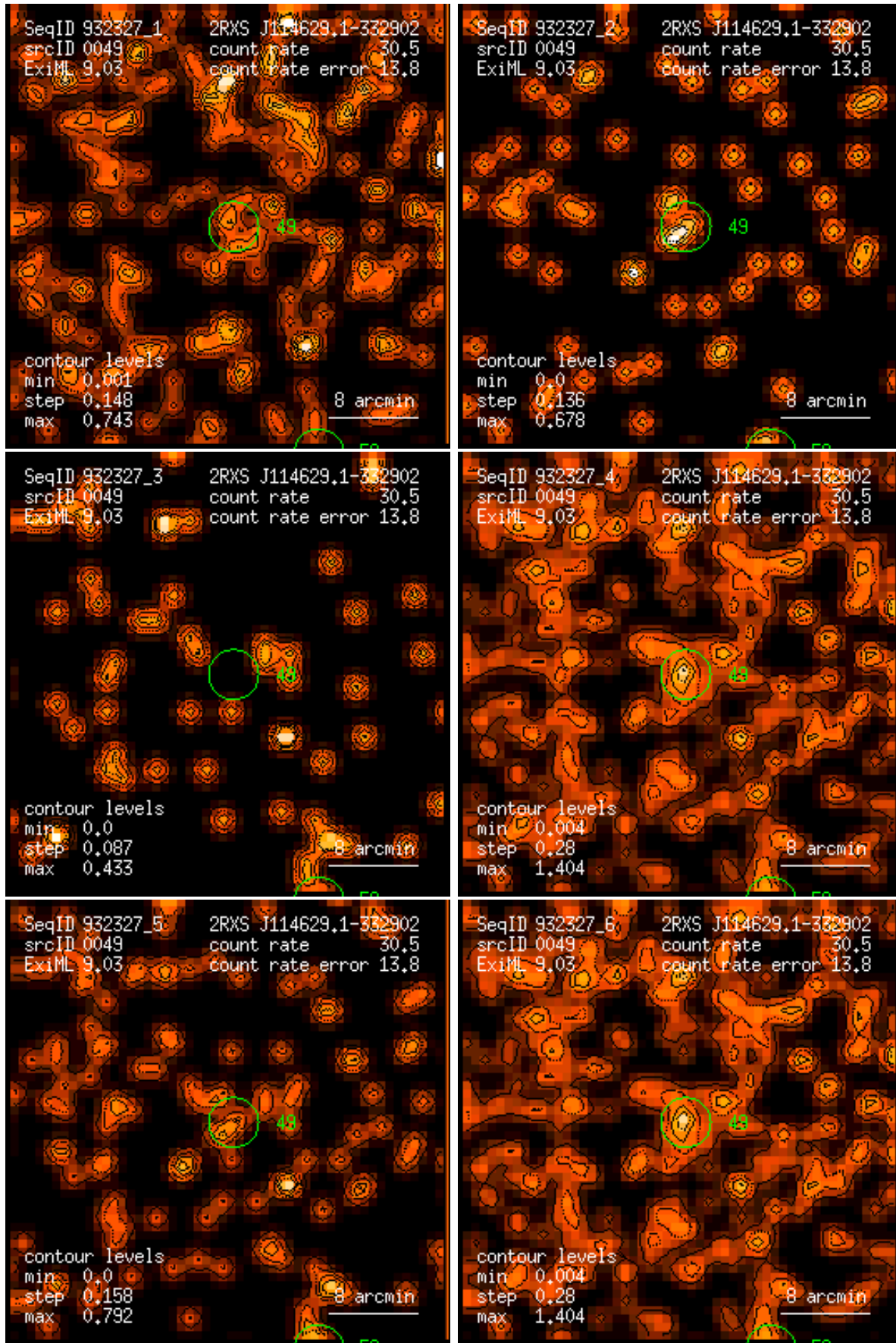
Figure 49: RASS 932327: detection 0049: band rate images, Gaussian filter: (1) PSPC channels 11 – 41, (2) 52 – 90, (3) 91 – 201, (4) 11 – 235, (5) 52 – 201, (6) 11 – 201. Broad band rates in counts/ks. Band rate contour levels in counts/ks/arcmin 2 .
