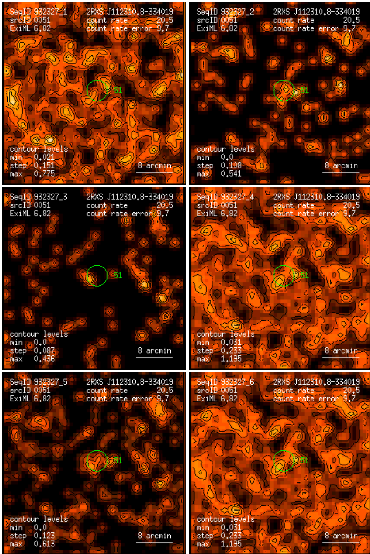
Figure 51: RASS 932327: detection 0051: band rate images, Gaussian filter: (1) PSPC channels 11 – 41, (2) 52 – 90, (3) 91 – 201, (4) 11 – 235, (5) 52 – 201, (6) 11 – 201. Broad band rates in counts/ks. Band rate contour levels in counts/ks/arcmin 2 .
