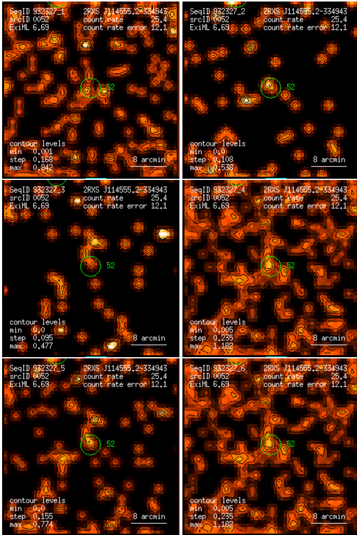
Figure 52: RASS 932327: detection 0052: band rate images, Gaussian filter: (1) PSPC channels 11 – 41, (2) 52 – 90, (3) 91 – 201, (4) 11 – 235, (5) 52 – 201, (6) 11 – 201. Broad band rates in counts/ks. Band rate contour levels in counts/ks/arcmin 2 .
