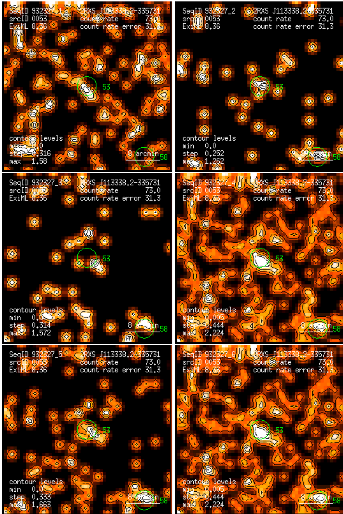
Figure 53: RASS 932327: detection 0053: band rate images, Gaussian filter: (1) PSPC channels 11 – 41, (2) 52 – 90, (3) 91 – 201, (4) 11 – 235, (5) 52 – 201, (6) 11 – 201. Broad band rates in counts/ks. Band rate contour levels in counts/ks/arcmin 2 .
