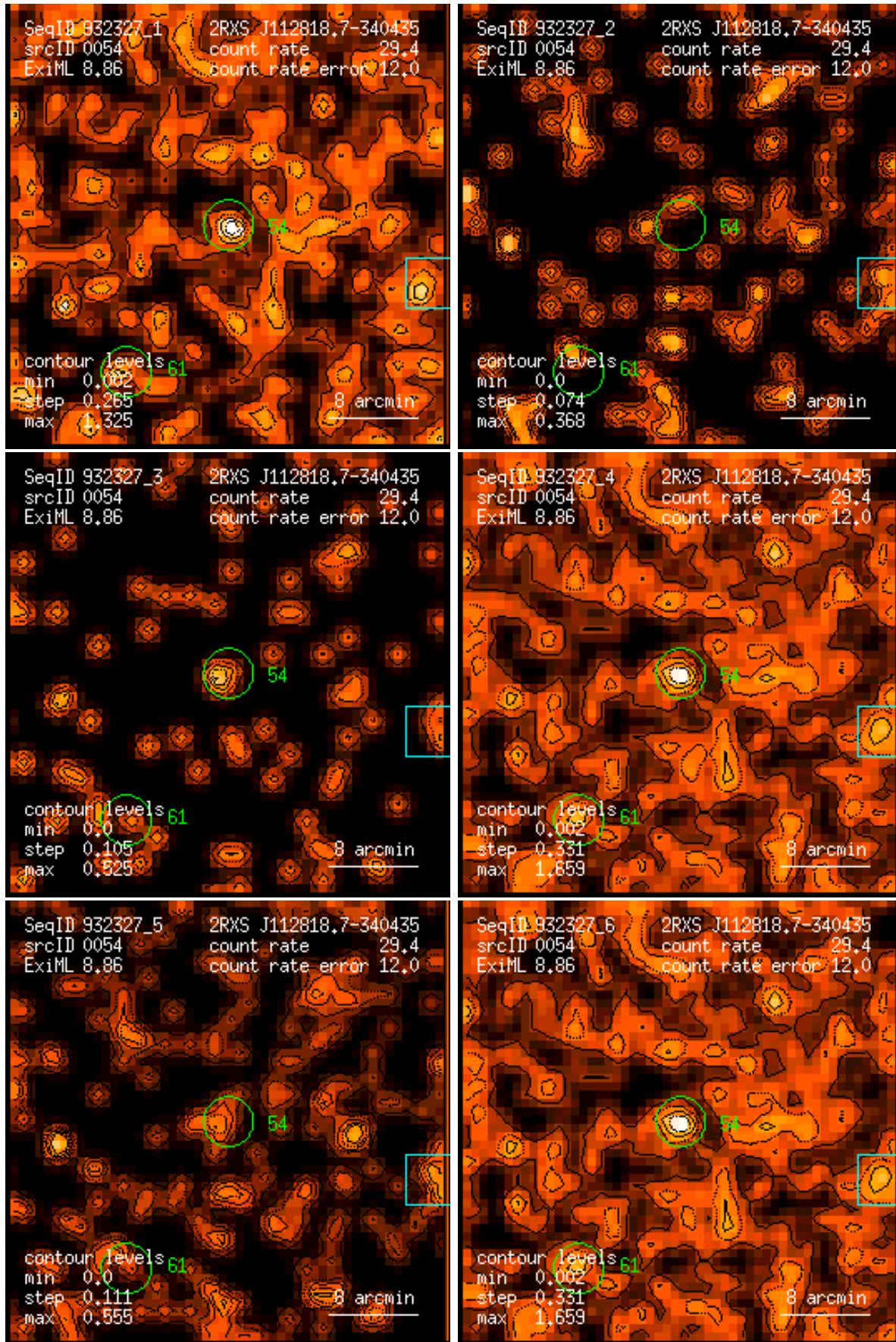
Figure 54: RASS 932327: detection 0054: band rate images, Gaussian filter: (1) PSPC channels 11 – 41, (2) 52 – 90, (3) 91 – 201, (4) 11 – 235, (5) 52 – 201, (6) 11 – 201. Broad band rates in counts/ks. Band rate contour levels in counts/ks/arcmin 2 .
