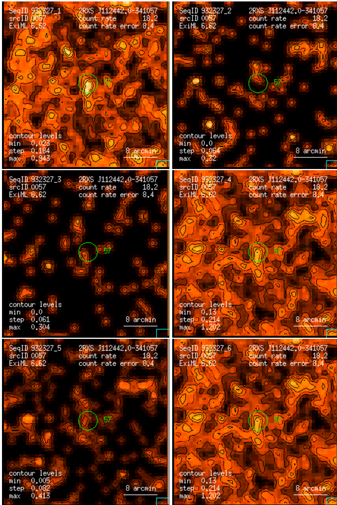
Figure 57: RASS 932327: detection 0057: band rate images, Gaussian filter: (1) PSPC channels 11 – 41, (2) 52 – 90, (3) 91 – 201, (4) 11 – 235, (5) 52 – 201, (6) 11 – 201. Broad band rates in counts/ks. Band rate contour levels in counts/ks/arcmin 2 .
