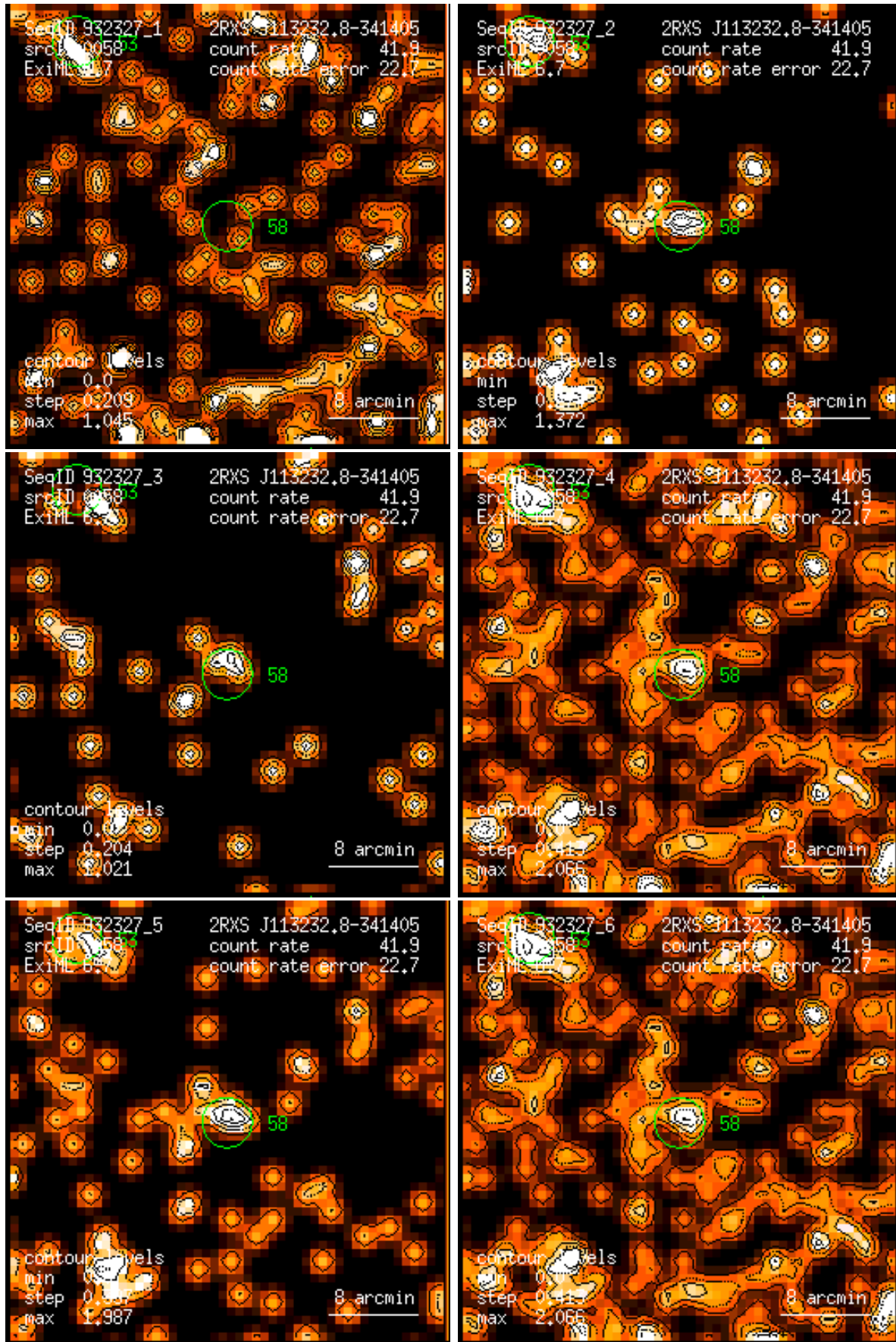
Figure 58: RASS 932327: detection 0058: band rate images, Gaussian filter: (1) PSPC channels 11 – 41, (2) 52 – 90, (3) 91 – 201, (4) 11 – 235, (5) 52 – 201, (6) 11 – 201. Broad band rates in counts/ks. Band rate contour levels in counts/ks/arcmin 2 .
