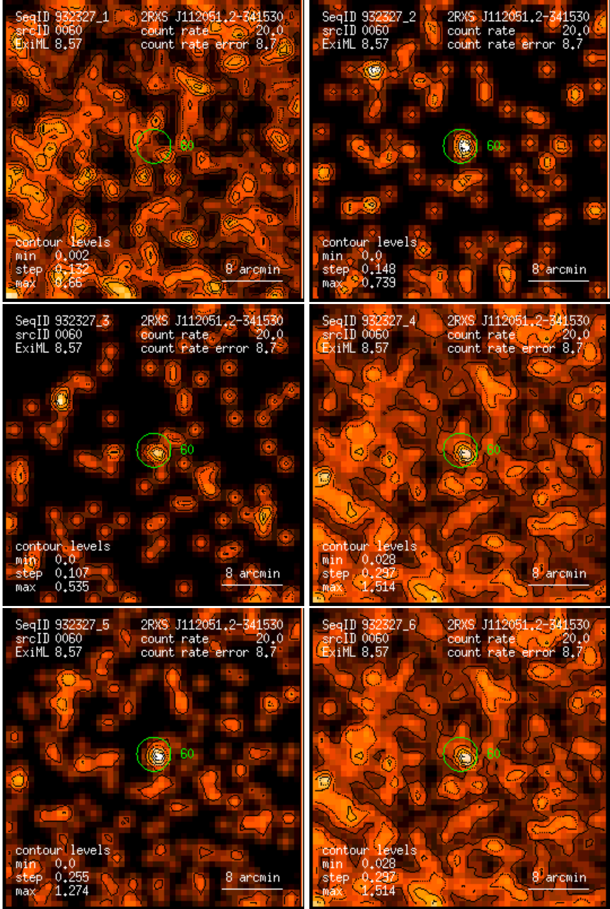
Figure 60: RASS 932327: detection 0060: band rate images, Gaussian filter: (1) PSPC channels 11 – 41, (2) 52 – 90, (3) 91 – 201, (4) 11 – 235, (5) 52 – 201, (6) 11 – 201. Broad band rates in counts/ks. Band rate contour levels in counts/ks/arcmin 2 .
