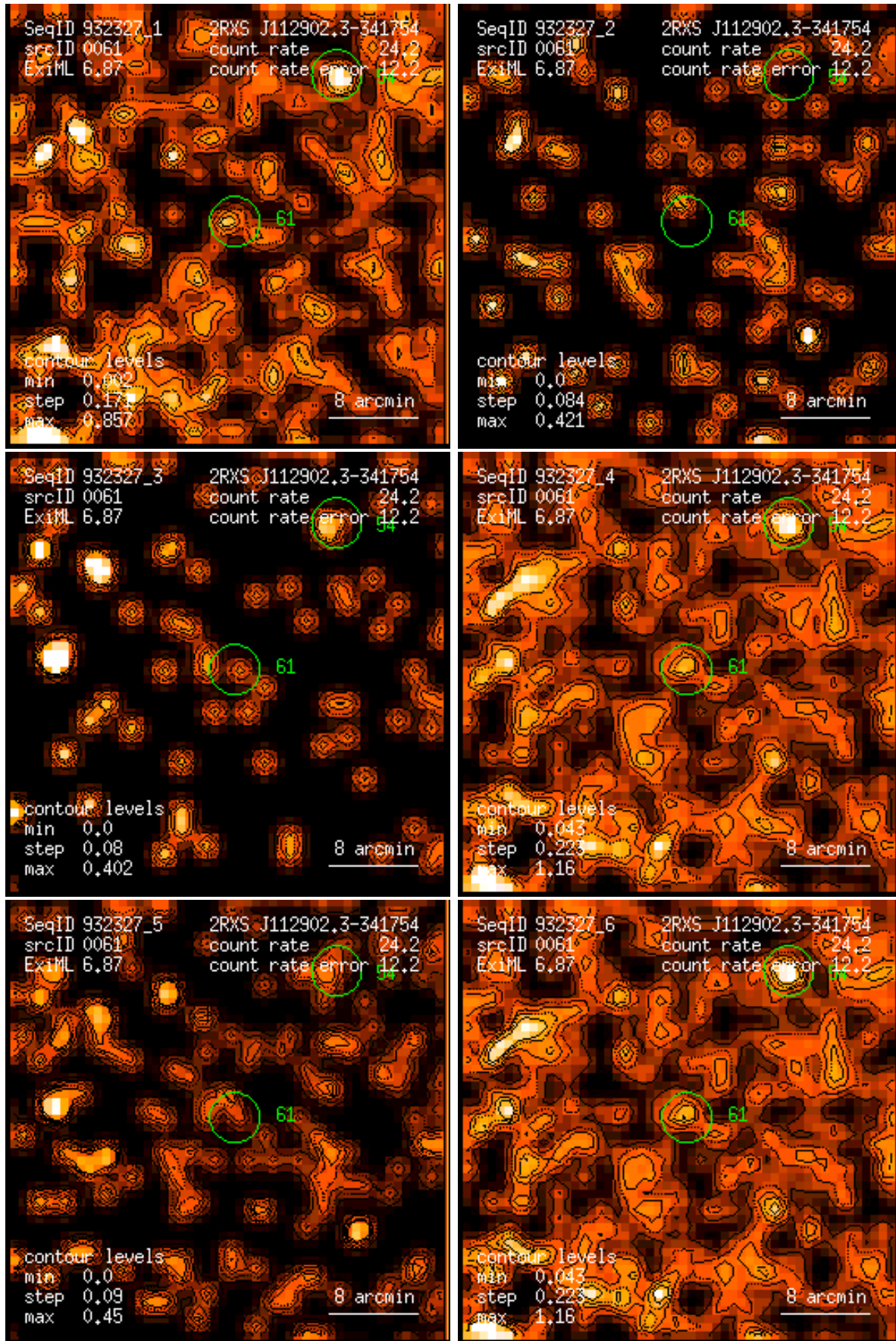
Figure 61: RASS 932327: detection 0061: band rate images, Gaussian filter: (1) PSPC channels 11 – 41, (2) 52 – 90, (3) 91 – 201, (4) 11 – 235, (5) 52 – 201, (6) 11 – 201. Broad band rates in counts/ks. Band rate contour levels in counts/ks/arcmin 2 .
