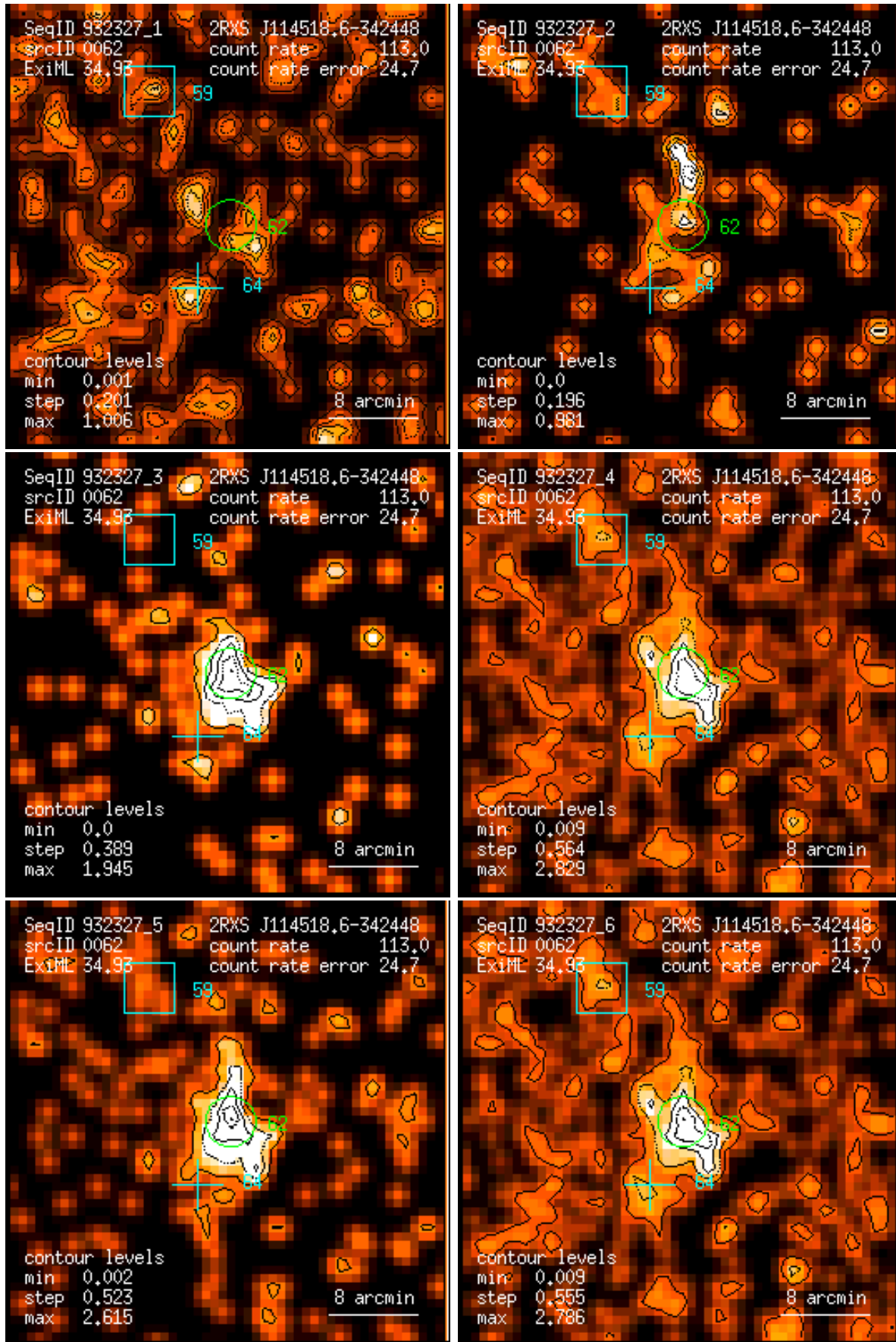
Figure 62: RASS 932327: detection 0062: band rate images, Gaussian filter: (1) PSPC channels 11 – 41, (2) 52 – 90, (3) 91 – 201, (4) 11 – 235, (5) 52 – 201, (6) 11 – 201. Broad band rates in counts/ks. Band rate contour levels in counts/ks/arcmin 2 .
