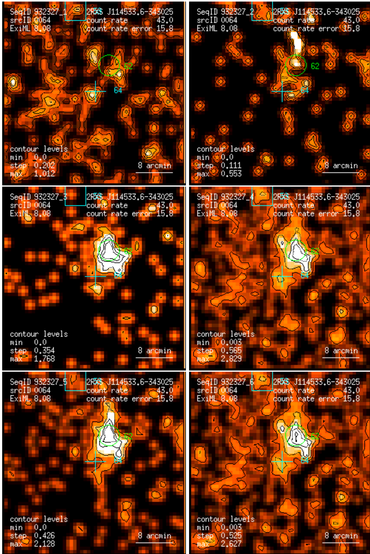
Figure 64: RASS 932327: detection 0064: band rate images, Gaussian filter: (1) PSPC channels 11 – 41, (2) 52 – 90, (3) 91 – 201, (4) 11 – 235, (5) 52 – 201, (6) 11 – 201. Broad band rates in counts/ks. Band rate contour levels in counts/ks/arcmin 2 .
