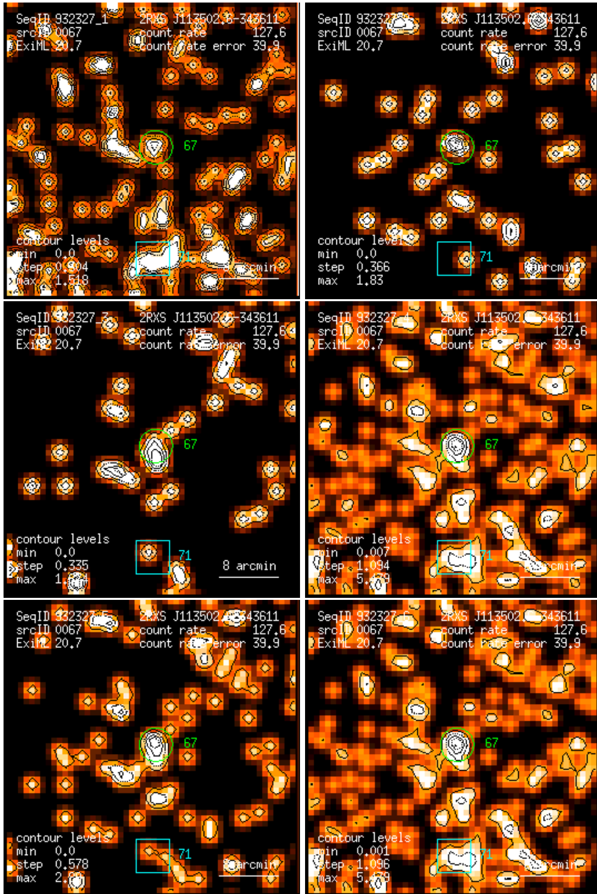
Figure 67: RASS 932327: detection 0067: band rate images, Gaussian filter: (1) PSPC channels 11 – 41, (2) 52 – 90, (3) 91 – 201, (4) 11 – 235, (5) 52 – 201, (6) 11 – 201. Broad band rates in counts/ks. Band rate contour levels in counts/ks/arcmin 2 .
