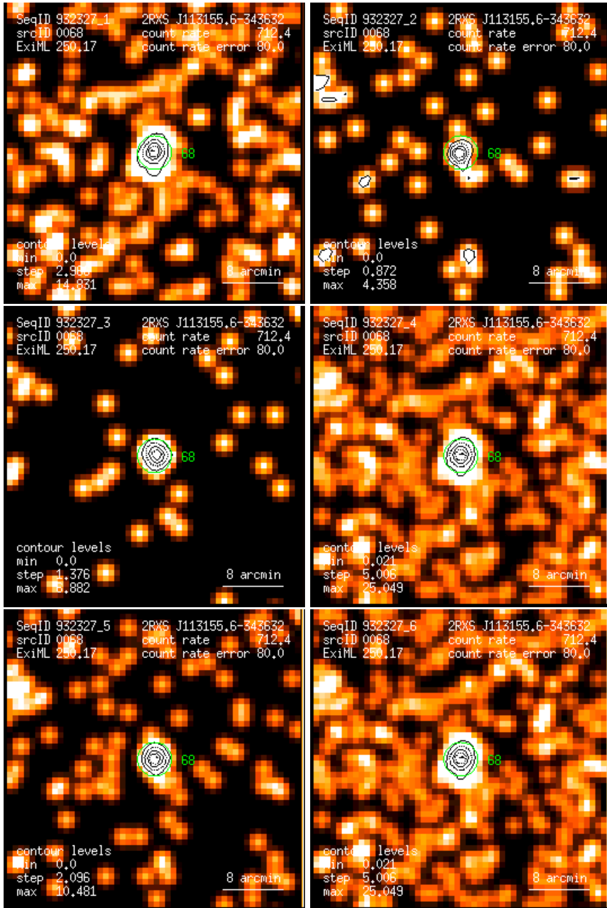
Figure 68: RASS 932327: detection 0068: band rate images, Gaussian filter: (1) PSPC channels 11 – 41, (2) 52 – 90, (3) 91 – 201, (4) 11 – 235, (5) 52 – 201, (6) 11 – 201. Broad band rates in counts/ks. Band rate contour levels in counts/ks/arcmin 2 .
