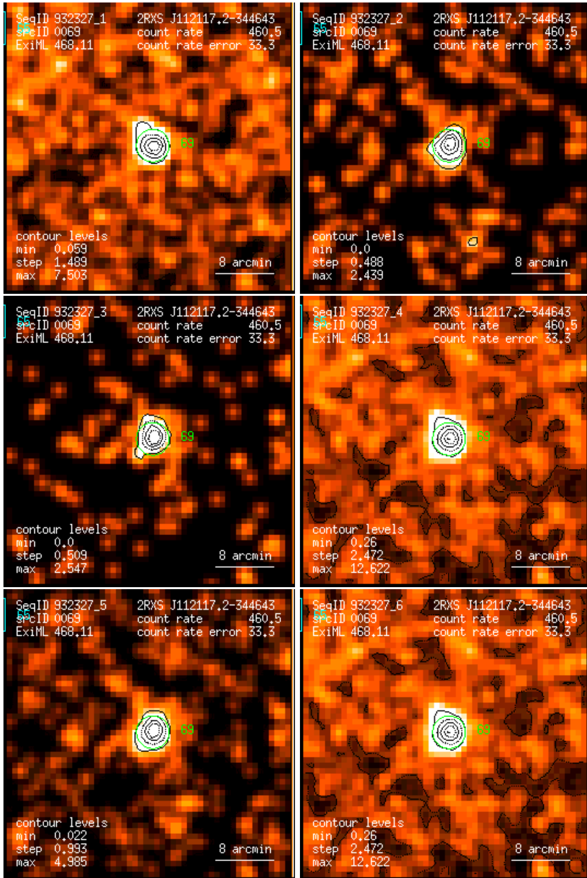
Figure 69: RASS 932327: detection 0069: band rate images, Gaussian filter: (1) PSPC channels 11 – 41, (2) 52 – 90, (3) 91 – 201, (4) 11 – 235, (5) 52 – 201, (6) 11 – 201. Broad band rates in counts/ks. Band rate contour levels in counts/ks/arcmin 2 .
