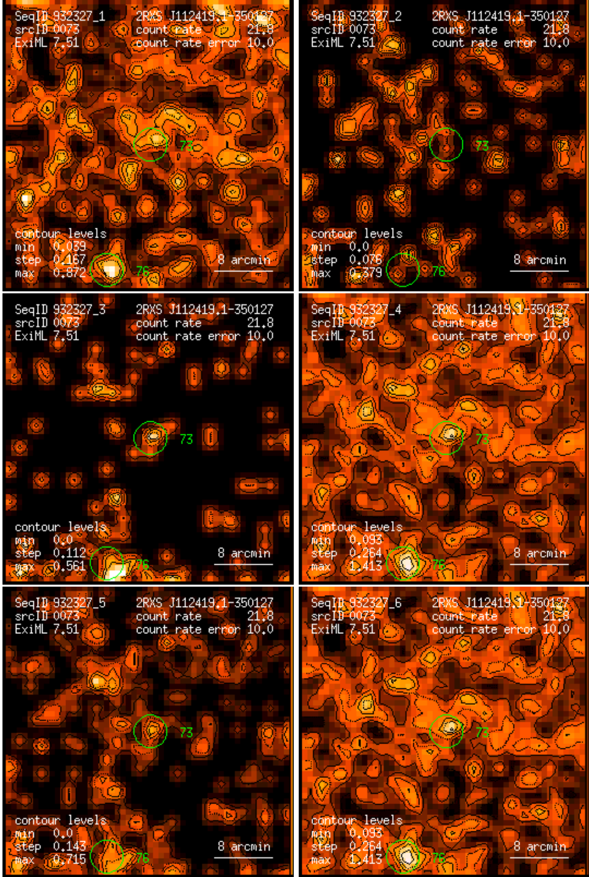
Figure 73: RASS 932327: detection 0073: band rate images, Gaussian filter: (1) PSPC channels 11 – 41, (2) 52 – 90, (3) 91 – 201, (4) 11 – 235, (5) 52 – 201, (6) 11 – 201. Broad band rates in counts/ks. Band rate contour levels in counts/ks/arcmin 2 .
