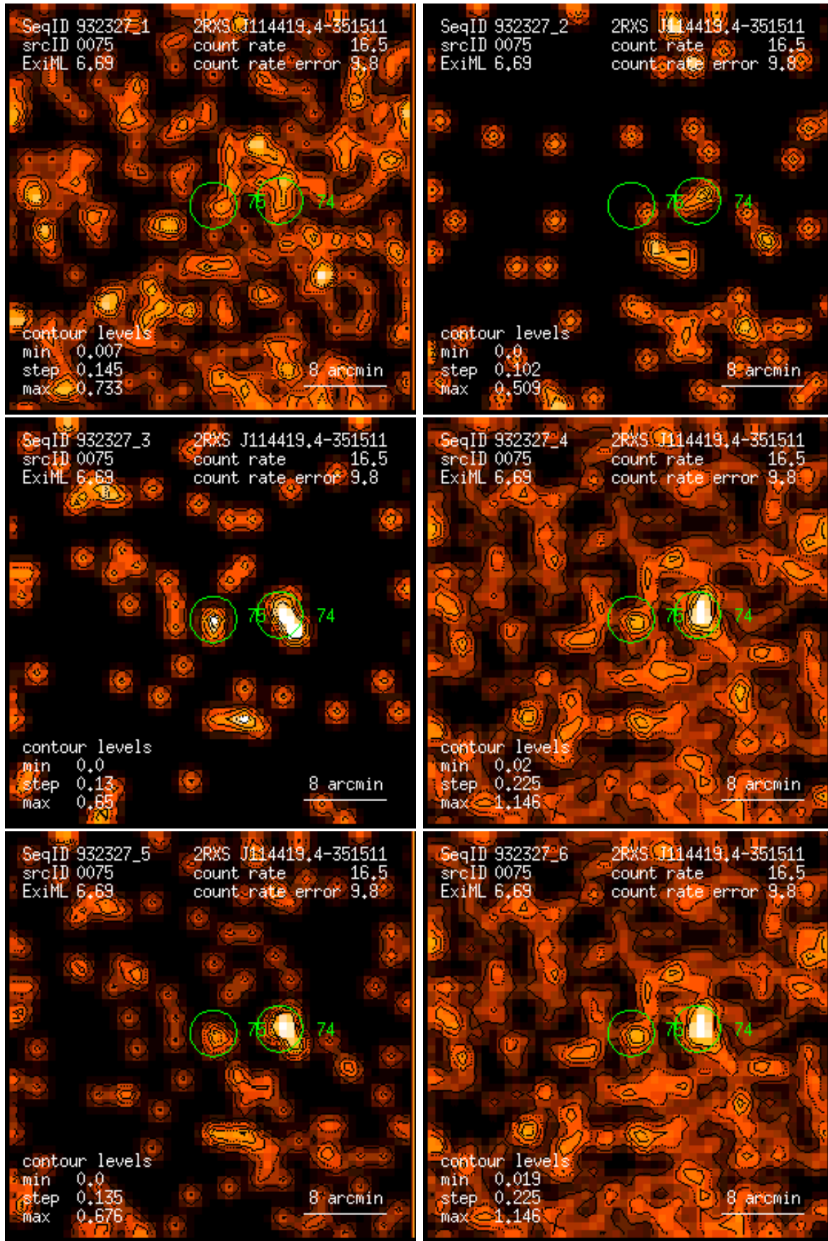
Figure 75: RASS 932327: detection 0075: band rate images, Gaussian filter: (1) PSPC channels 11 – 41, (2) 52 – 90, (3) 91 – 201, (4) 11 – 235, (5) 52 – 201, (6) 11 – 201. Broad band rates in counts/ks. Band rate contour levels in counts/ks/arcmin 2 .
