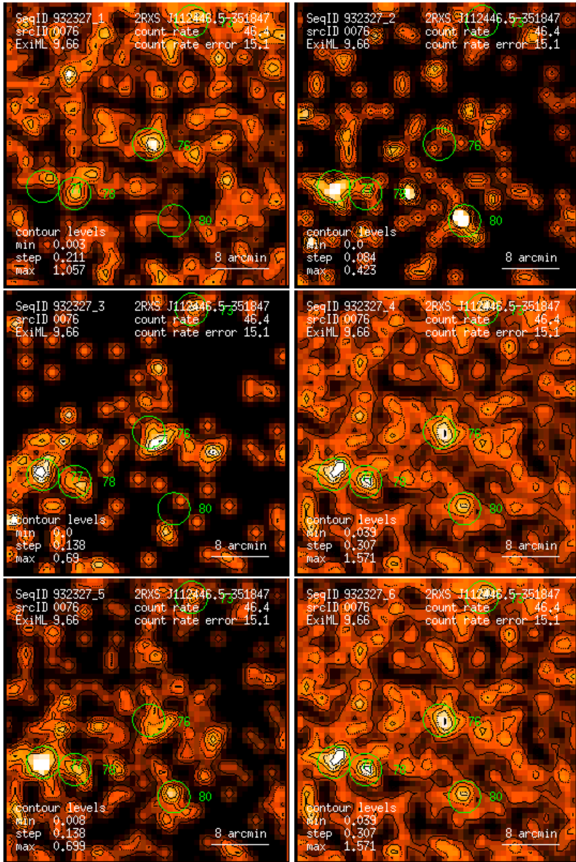
Figure 76: RASS 932327: detection 0076: band rate images, Gaussian filter: (1) PSPC channels 11 – 41, (2) 52 – 90, (3) 91 – 201, (4) 11 – 235, (5) 52 – 201, (6) 11 – 201. Broad band rates in counts/ks. Band rate contour levels in counts/ks/arcmin 2 .
