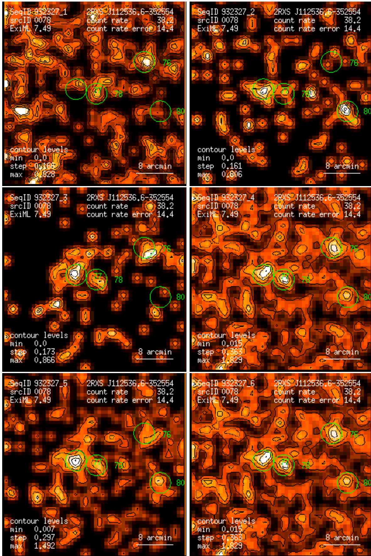
Figure 78: RASS 932327: detection 0078: band rate images, Gaussian filter: (1) PSPC channels 11 – 41, (2) 52 – 90, (3) 91 – 201, (4) 11 – 235, (5) 52 – 201, (6) 11 – 201. Broad band rates in counts/ks. Band rate contour levels in counts/ks/arcmin 2 .
