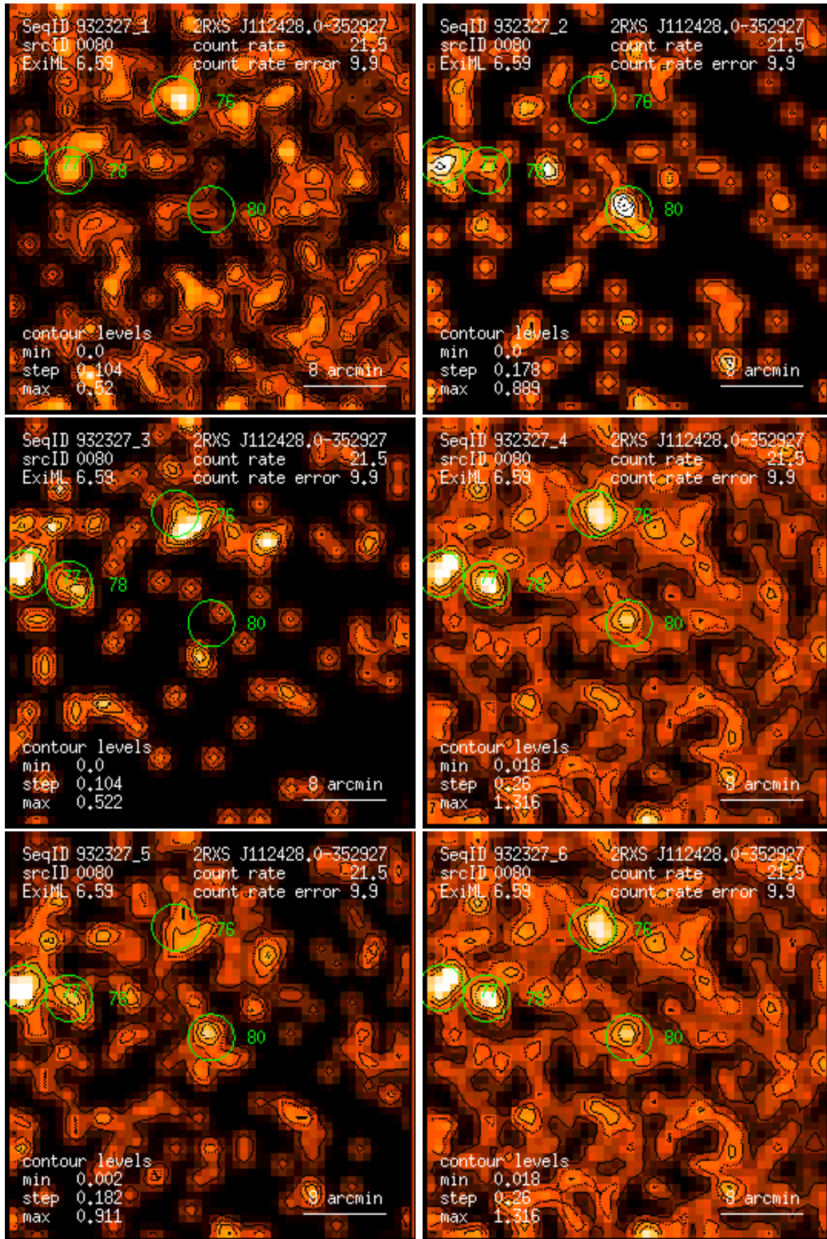
Figure 80: RASS 932327: detection 0080: band rate images, Gaussian filter: (1) PSPC channels 11 – 41, (2) 52 – 90, (3) 91 – 201, (4) 11 – 235, (5) 52 – 201, (6) 11 – 201. Broad band rates in counts/ks. Band rate contour levels in counts/ks/arcmin 2 .
