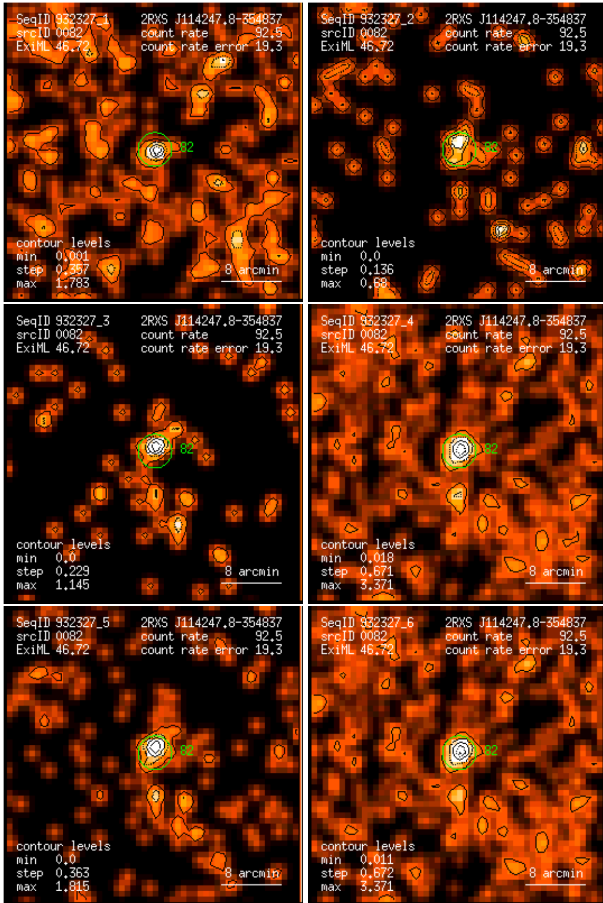
Figure 82: RASS 932327: detection 0082: band rate images, Gaussian filter: (1) PSPC channels 11 – 41, (2) 52 – 90, (3) 91 – 201, (4) 11 – 235, (5) 52 – 201, (6) 11 – 201. Broad band rates in counts/ks. Band rate contour levels in counts/ks/arcmin 2 .
