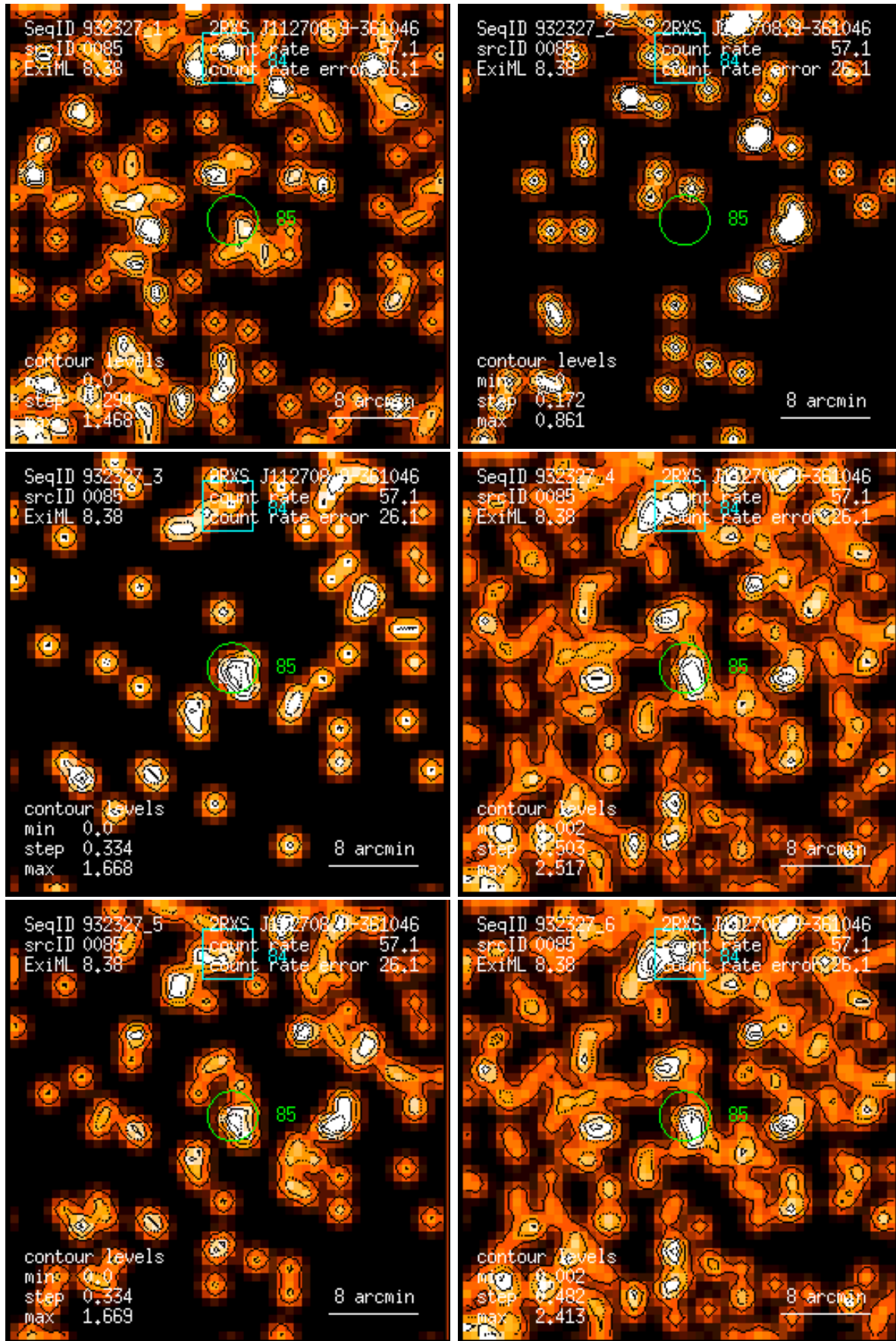
Figure 85: RASS 932327: detection 0085: band rate images, Gaussian filter: (1) PSPC channels 11 – 41, (2) 52 – 90, (3) 91 – 201, (4) 11 – 235, (5) 52 – 201, (6) 11 – 201. Broad band rates in counts/ks. Band rate contour levels in counts/ks/arcmin 2 .
