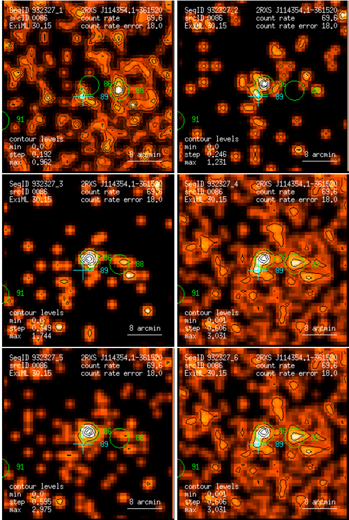
Figure 86: RASS 932327: detection 0086: band rate images, Gaussian filter: (1) PSPC channels 11 – 41, (2) 52 – 90, (3) 91 – 201, (4) 11 – 235, (5) 52 – 201, (6) 11 – 201. Broad band rates in counts/ks. Band rate contour levels in counts/ks/arcmin 2 .
