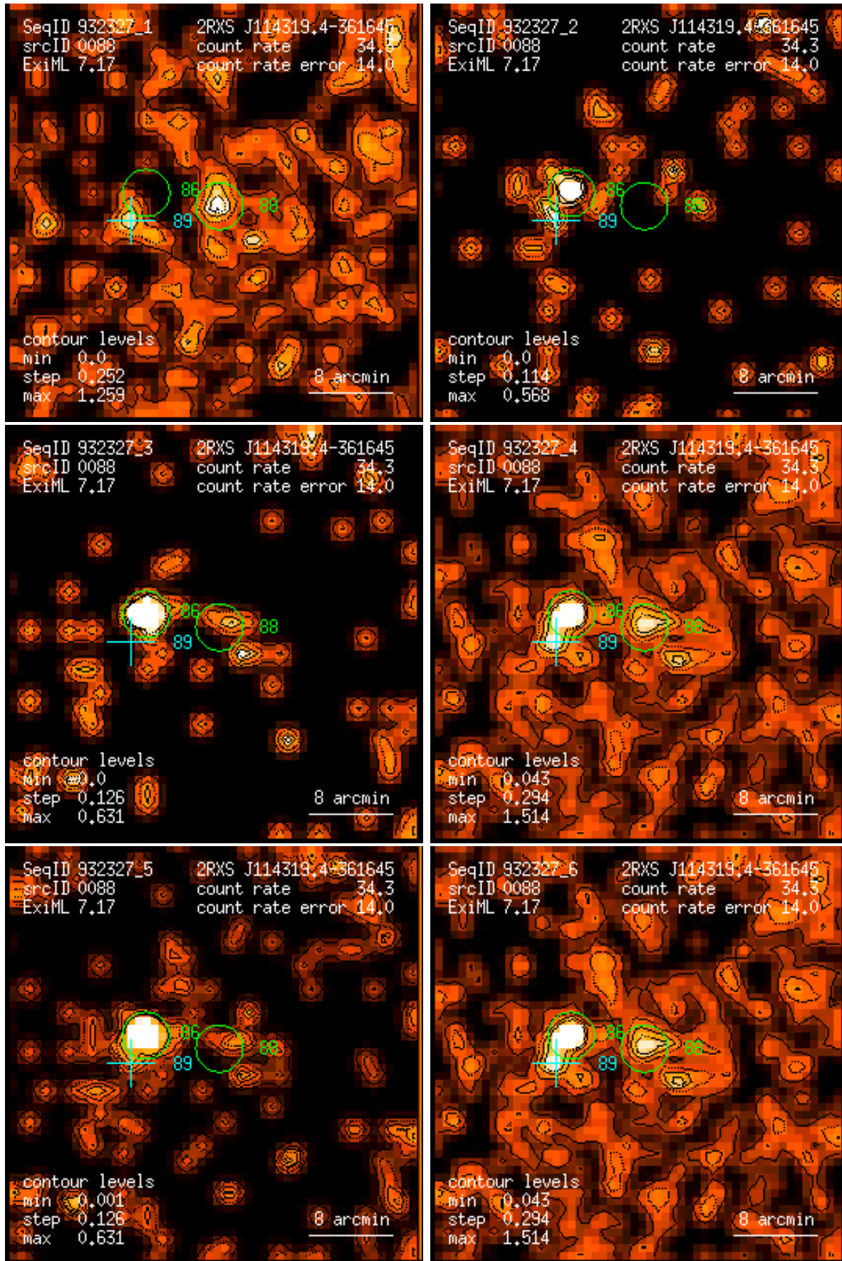
Figure 88: RASS 932327: detection 0088: band rate images, Gaussian filter: (1) PSPC channels 11 – 41, (2) 52 – 90, (3) 91 – 201, (4) 11 – 235, (5) 52 – 201, (6) 11 – 201. Broad band rates in counts/ks. Band rate contour levels in counts/ks/arcmin 2 .
