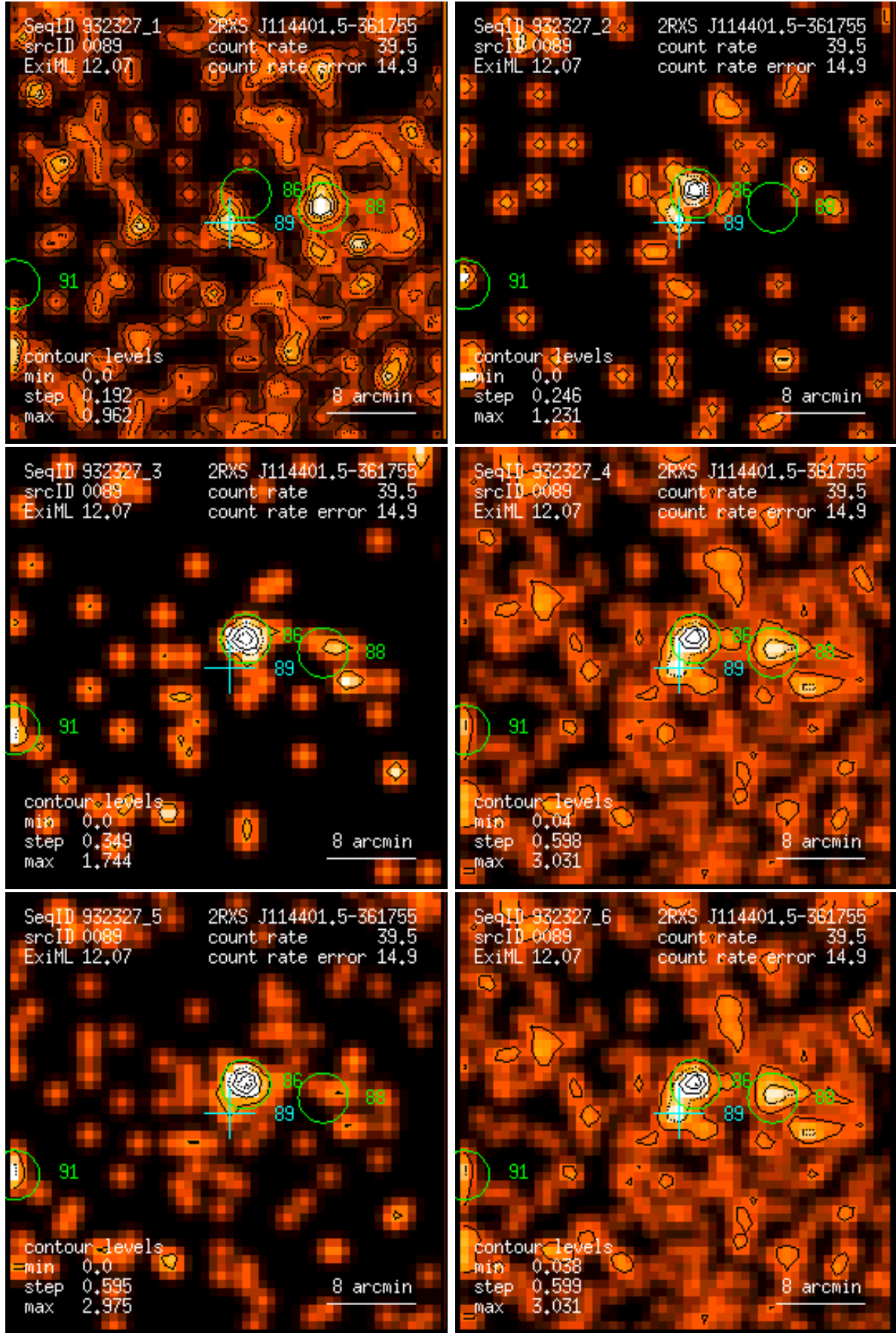
Figure 89: RASS 932327: detection 0089: band rate images, Gaussian filter: (1) PSPC channels 11 – 41, (2) 52 – 90, (3) 91 – 201, (4) 11 – 235, (5) 52 – 201, (6) 11 – 201. Broad band rates in counts/ks. Band rate contour levels in counts/ks/arcmin 2 .
