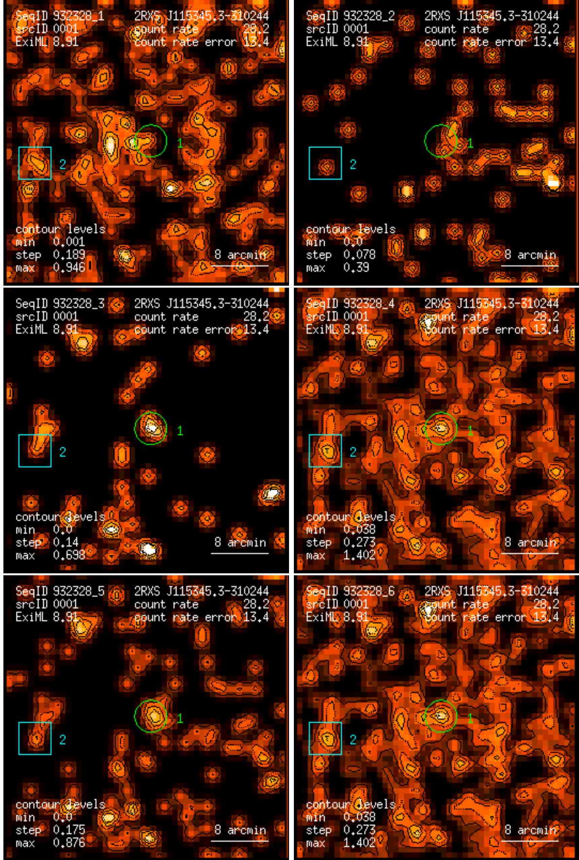
Figure 1: RASS 932328: detection 0001: band rate images, Gaussian filter: (1) PSPC channels 11 – 41, (2) 52 – 90, (3) 91 – 201, (4) 11 – 235, (5) 52 – 201, (6) 11 – 201. Broad band rates in counts/ks. Band rate contour levels in counts/ks/arcmin 2 .
