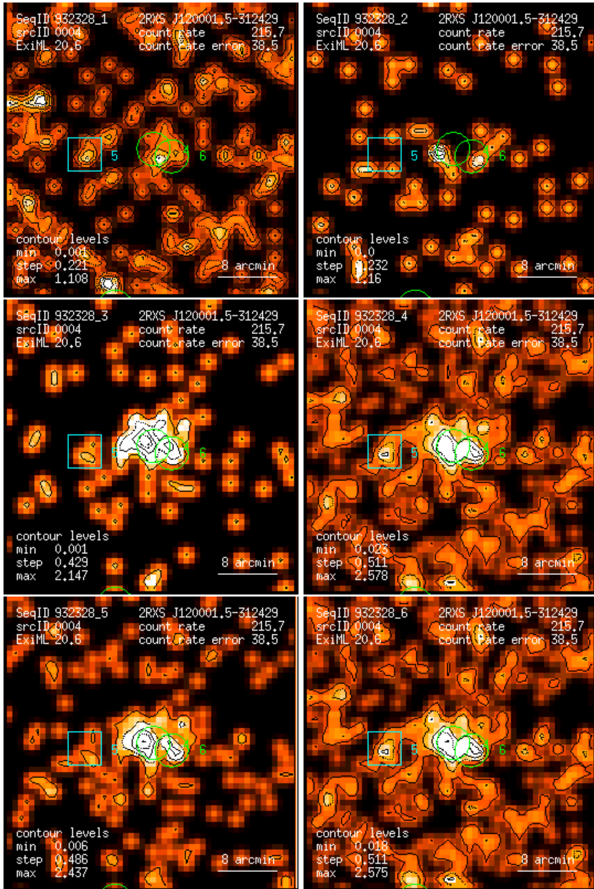
Figure 4: RASS 932328: detection 0004: band rate images, Gaussian filter: (1) PSPC channels 11 – 41, (2) 52 – 90, (3) 91 – 201, (4) 11 – 235, (5) 52 – 201, (6) 11 – 201. Broad band rates in counts/ks. Band rate contour levels in counts/ks/arcmin 2 .
