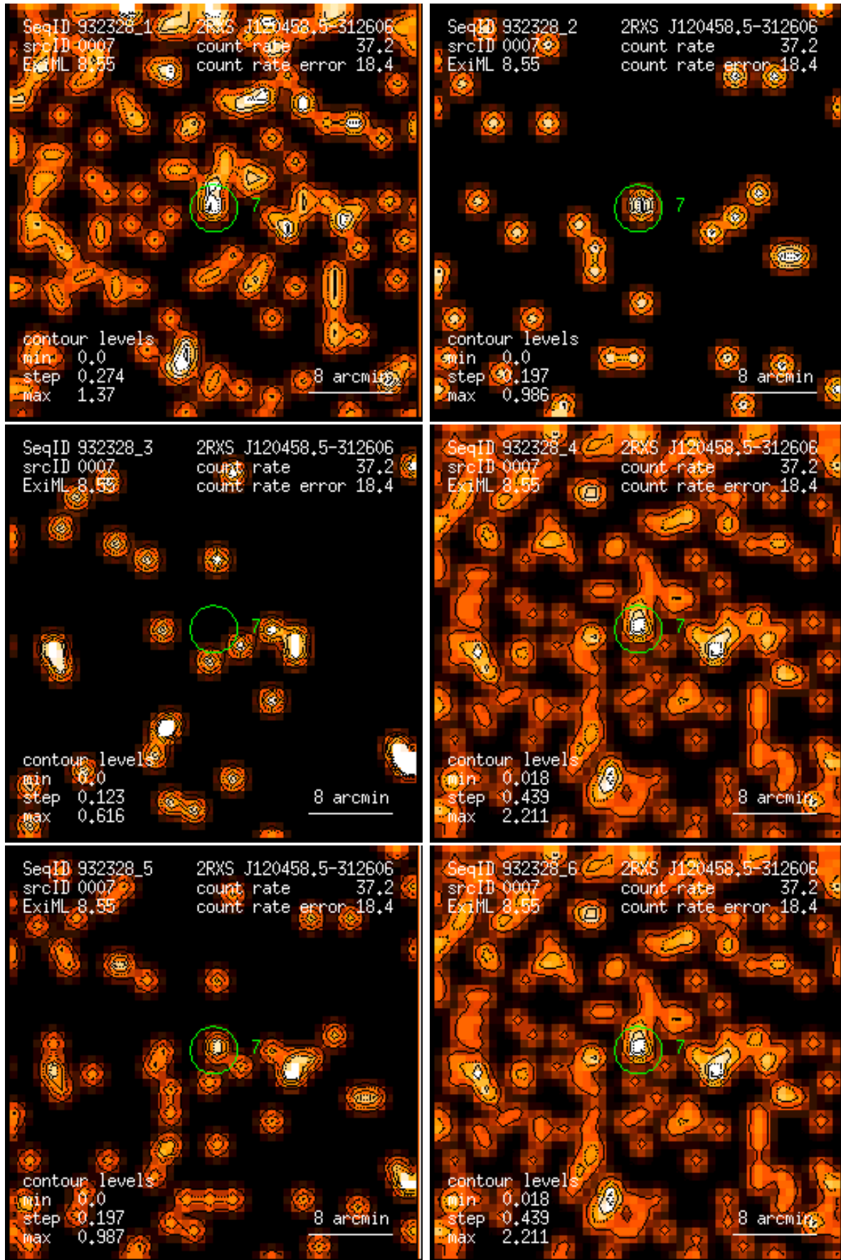
Figure 7: RASS 932328: detection 0007: band rate images, Gaussian filter: (1) PSPC channels 11 – 41, (2) 52 – 90, (3) 91 – 201, (4) 11 – 235, (5) 52 – 201, (6) 11 – 201. Broad band rates in counts/ks. Band rate contour levels in counts/ks/arcmin 2 .
