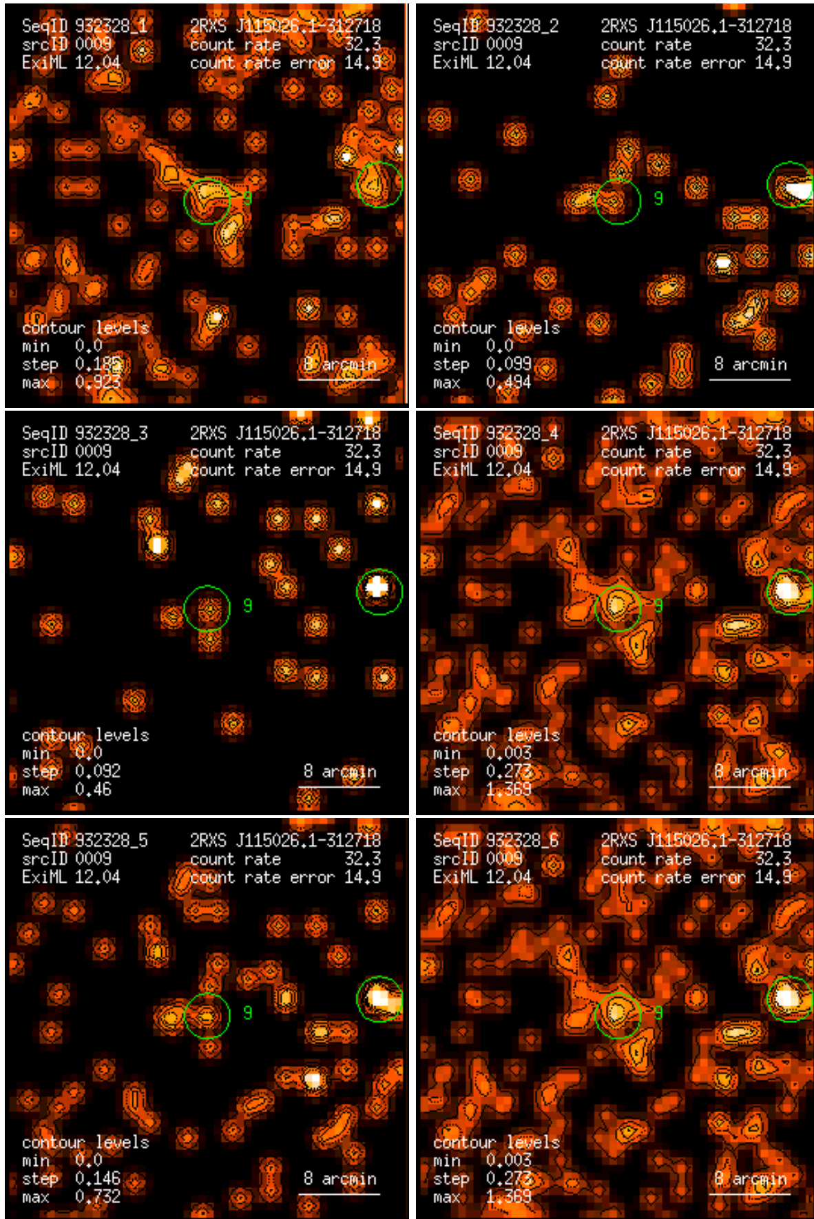
Figure 9: RASS 932328: detection 0009: band rate images, Gaussian filter: (1) PSPC channels 11 – 41, (2) 52 – 90, (3) 91 – 201, (4) 11 – 235, (5) 52 – 201, (6) 11 – 201. Broad band rates in counts/ks. Band rate contour levels in counts/ks/arcmin 2 .
