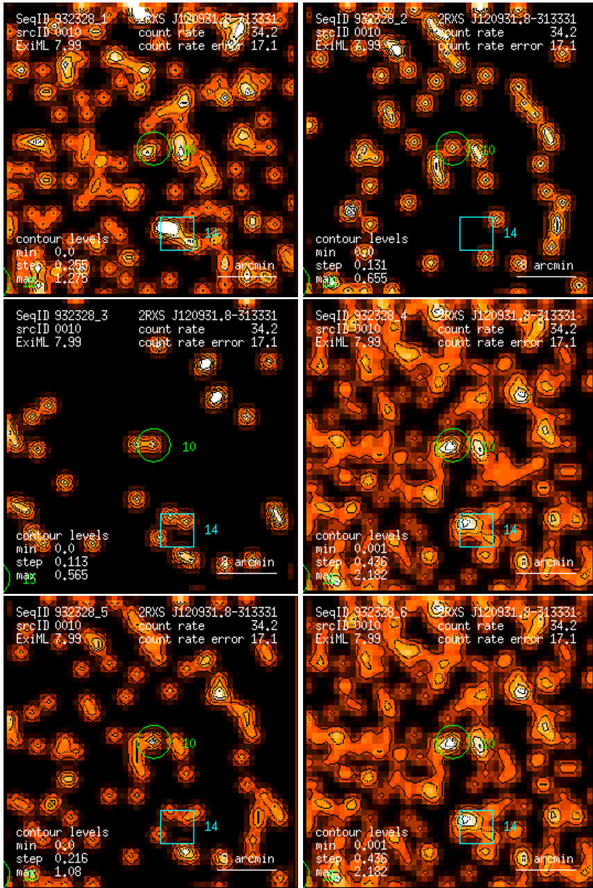
Figure 10: RASS 932328: detection 0010: band rate images, Gaussian filter: (1) PSPC channels 11 – 41, (2) 52 – 90, (3) 91 – 201, (4) 11 – 235, (5) 52 – 201, (6) 11 – 201. Broad band rates in counts/ks. Band rate contour levels in counts/ks/arcmin 2 .
